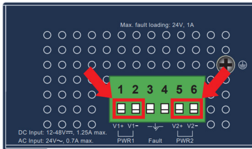
Figure 3-1: IGS-10020MT Upper Panel
