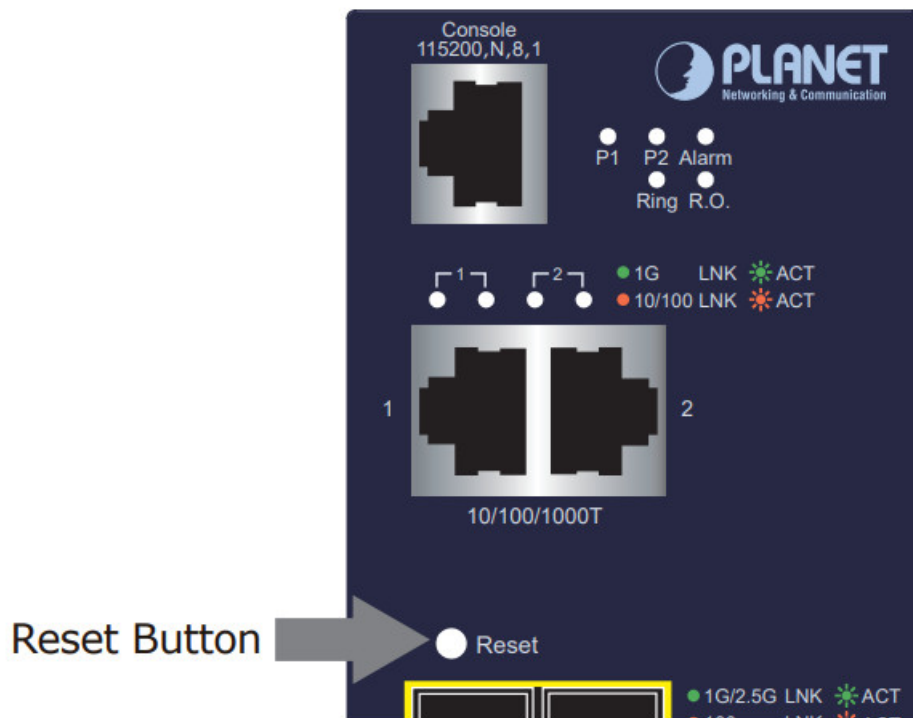
Figure 6-2: IGS-10080MFT Reset Button
