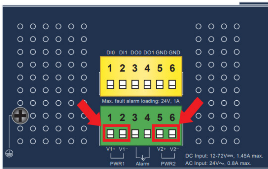
Figure 3-3: IGS-12040MT Upper Panel
