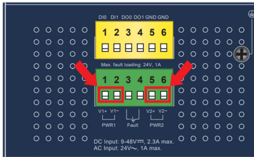
Figure 3-4: IGS-20040MT Upper Panel
