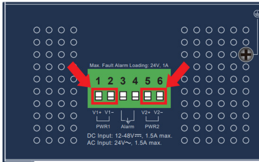
Figure 3-2: IGS-10080MFT Upper Panel
