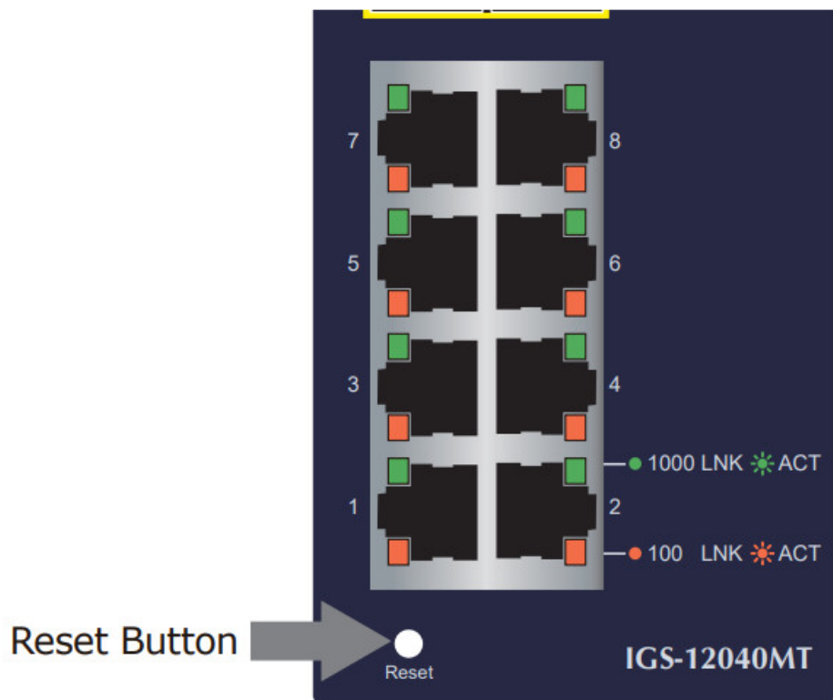
Figure 6-3: IGS-12040MT Reset Button
