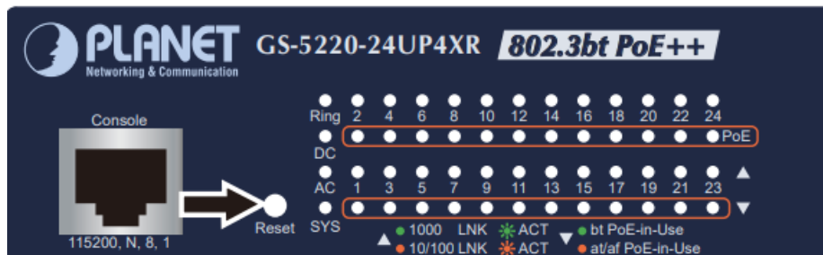
Figure 5-2: GS-5220-24UP4X(R) Reset Button
