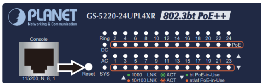
Figure 5-3: GS-5220-24UPL4X(R) Reset Button
