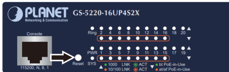
Figure 5-1: GS-5220-16UP4S2X(R) Reset Button
