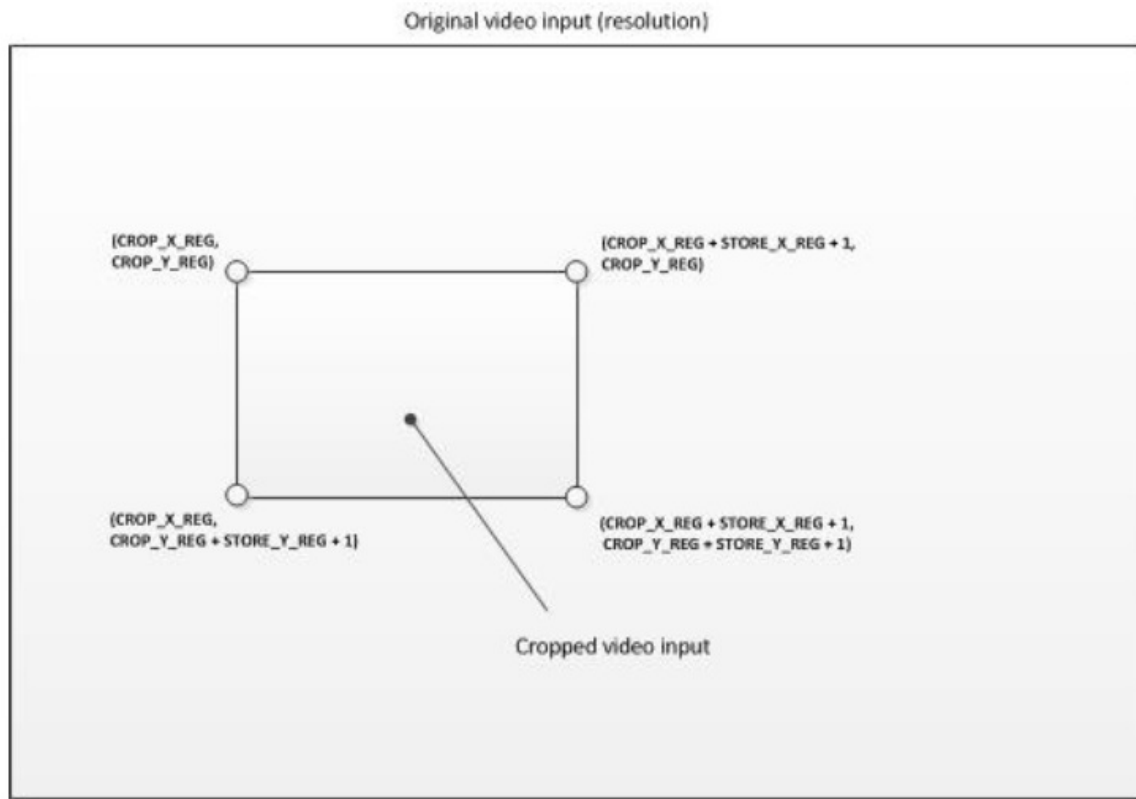
Figure 3. Explanation of Video Input Cropping
