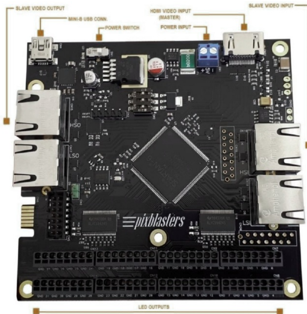
Figure 2. Board's Terminals Important for the Initialization Process
