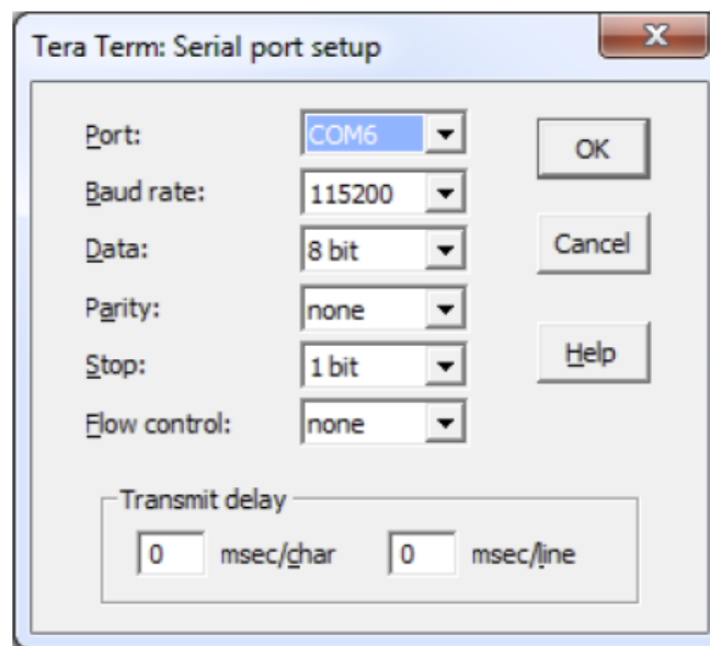
Figure 7. Correct Serial Connection Parameters
