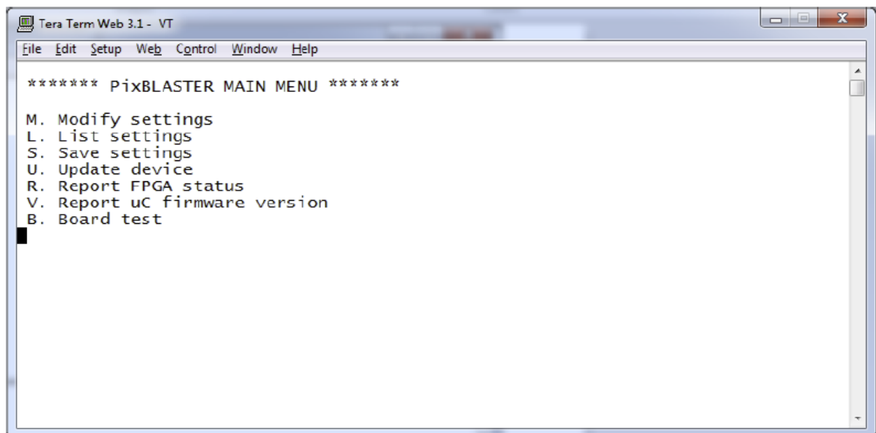
Figure 14. The Main Menu in Configuration 0
