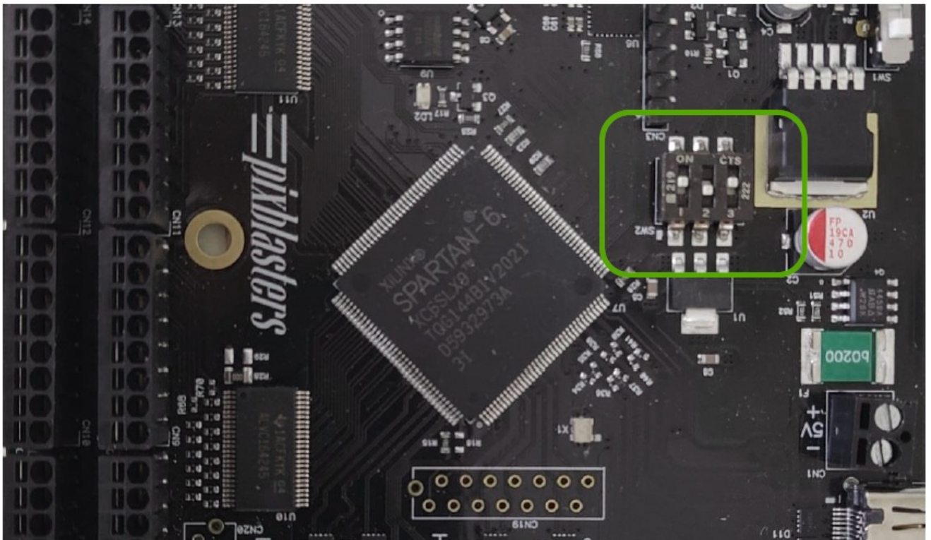
Figure 6. On-Board DIP Switches Set To Master Configuration*
