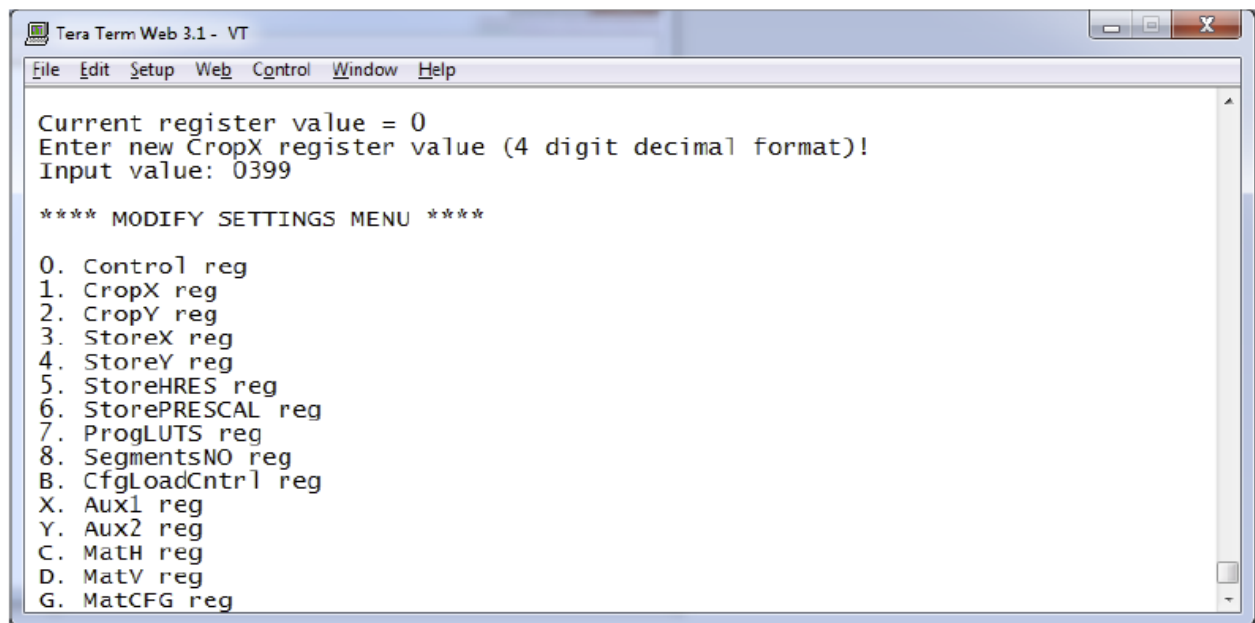
Figure 10. Example Modification of Internal Registers
