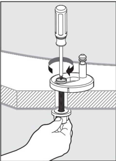
Option B: Tighten the bolts [D] further while holding the nuts [E] underneath.
