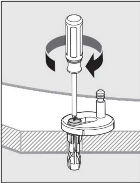
Option A: Fully tighten the bolts [D]
