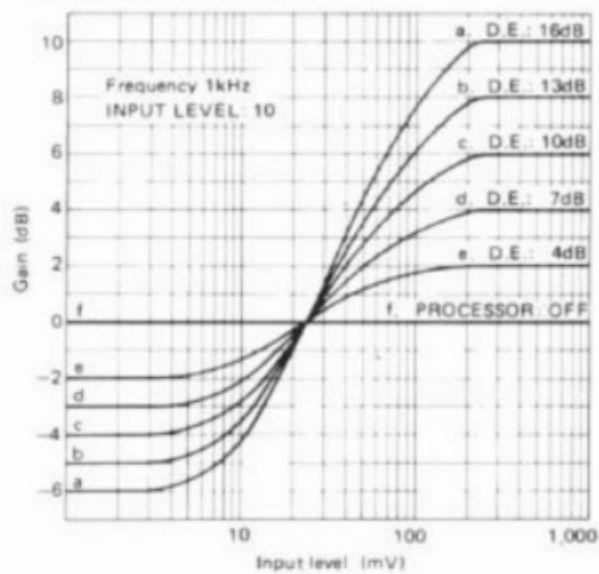
Fig. 6: RG processor input-gain characteristics
