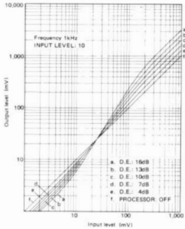
Fig. 5: RG processor input-output transfer characteristics
