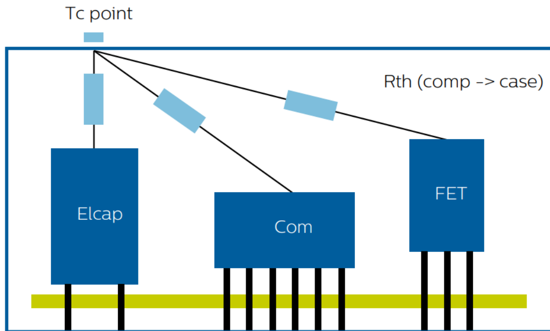
Schematical representation of internal thermal paths to the SR Bridge t_c point
