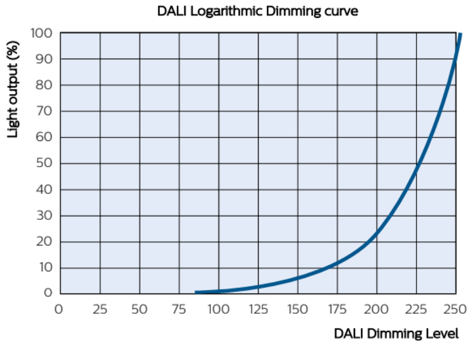
DALI Logarithmic dimming curve
