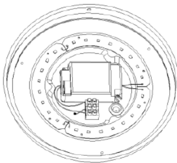
LIGHT SOURCE
