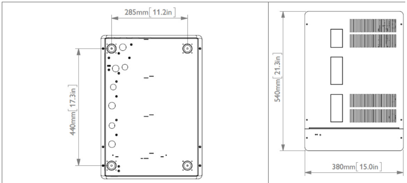
Enclosure diagram
