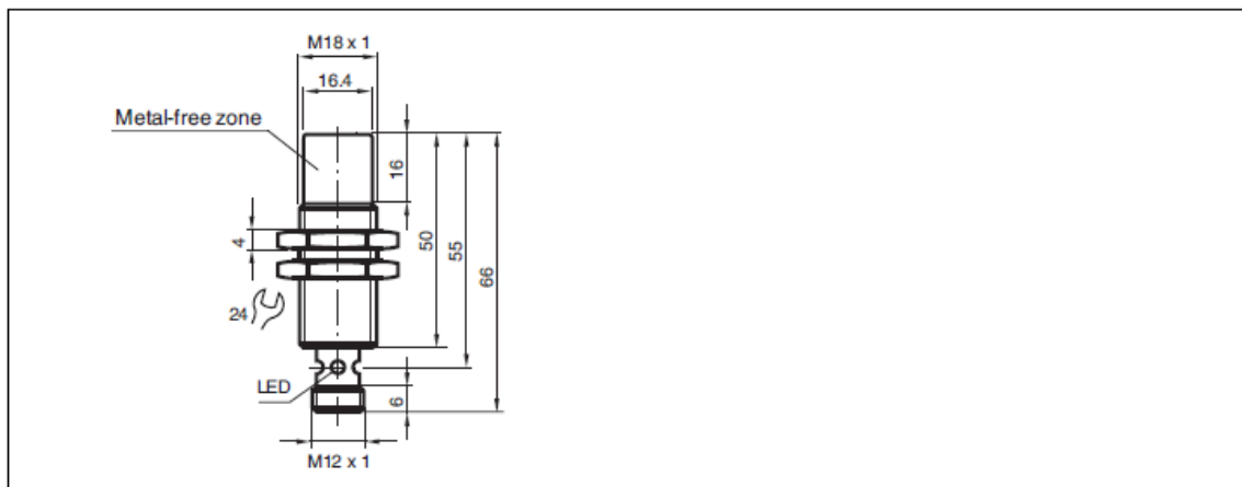
Figure 3.6 IQH1-18GM-V1
