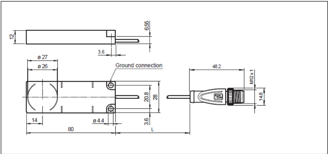
Figure 3.5 IQH1-F61-V1
