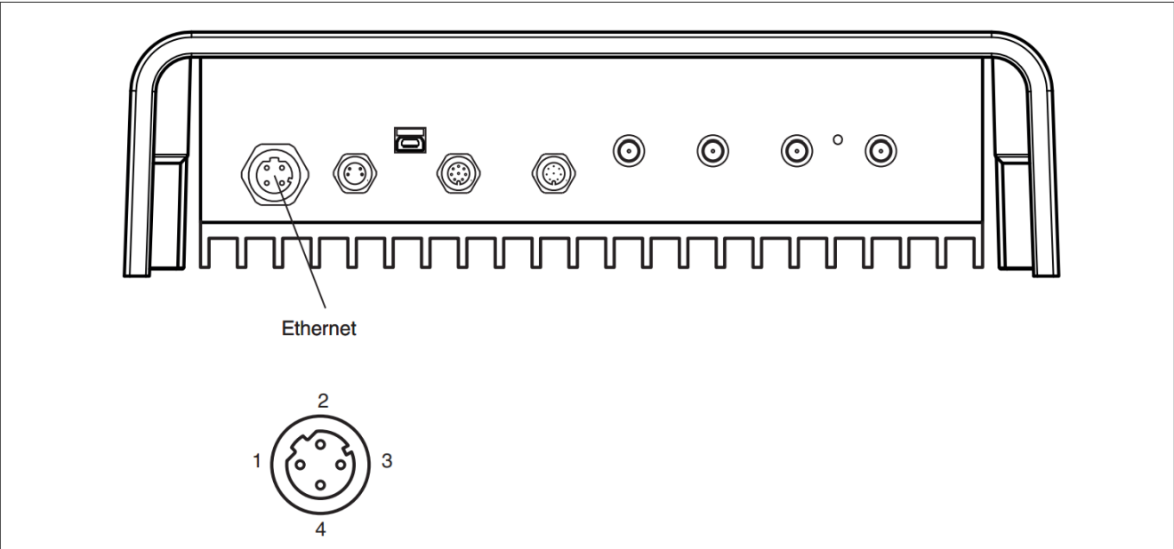
Figure 4.4 Pinout
