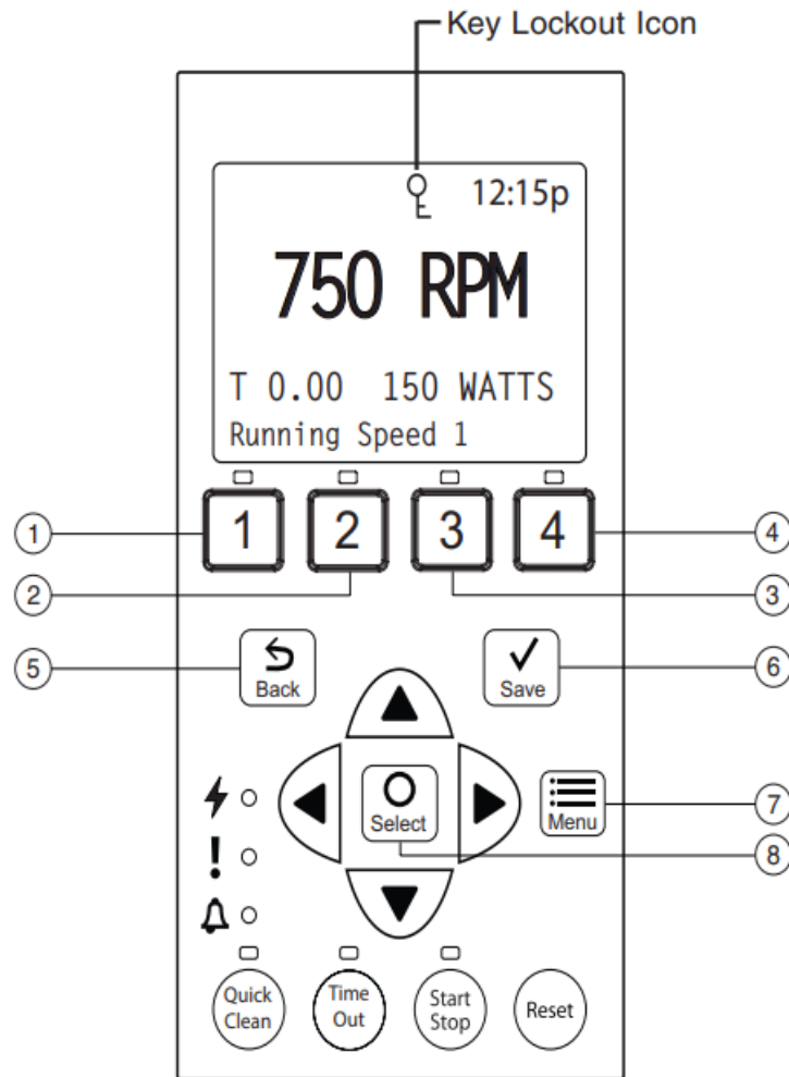
Control Panel #1-8
