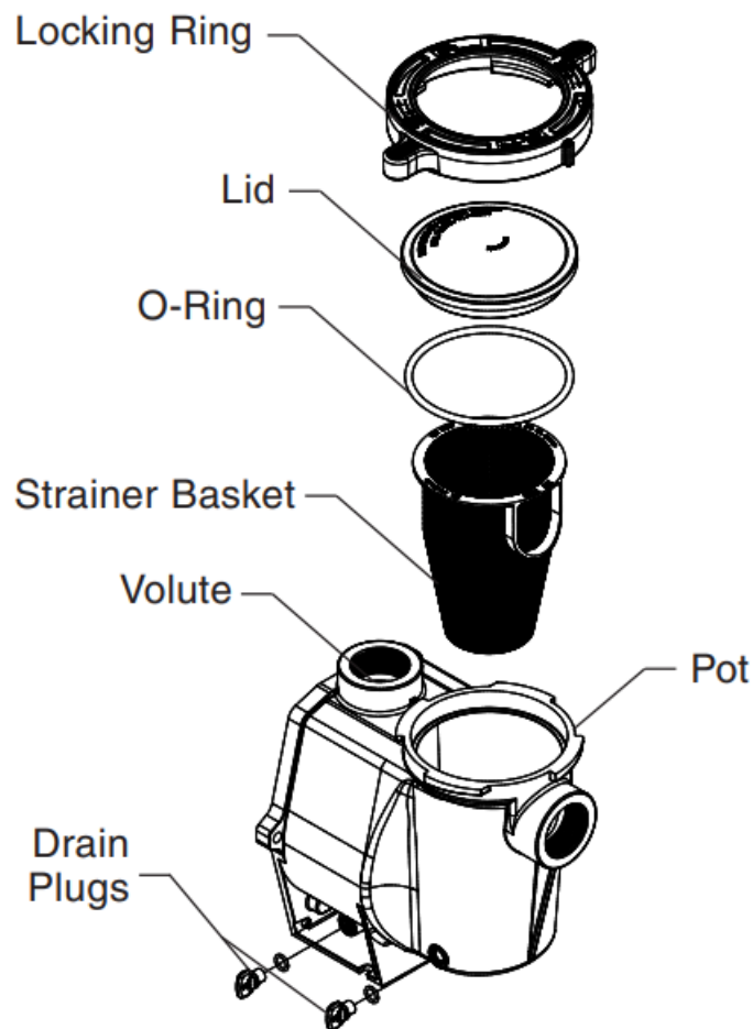
Strainer Pot Assembly
