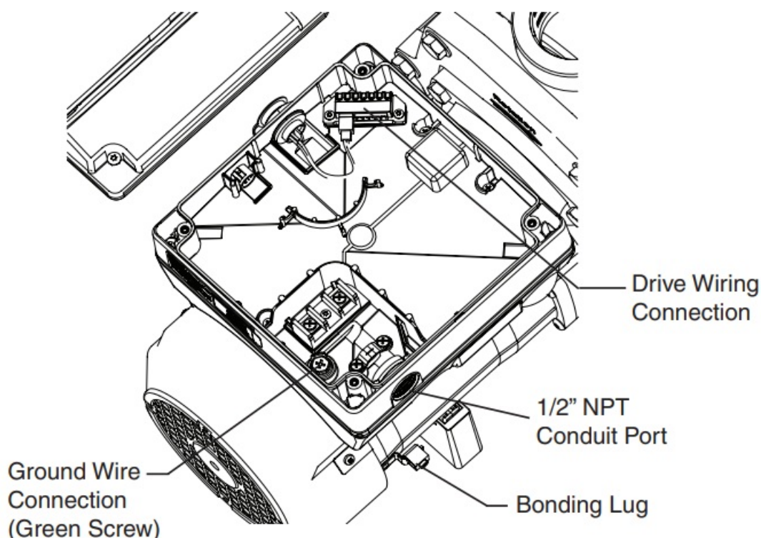
Field Wiring Compartment
