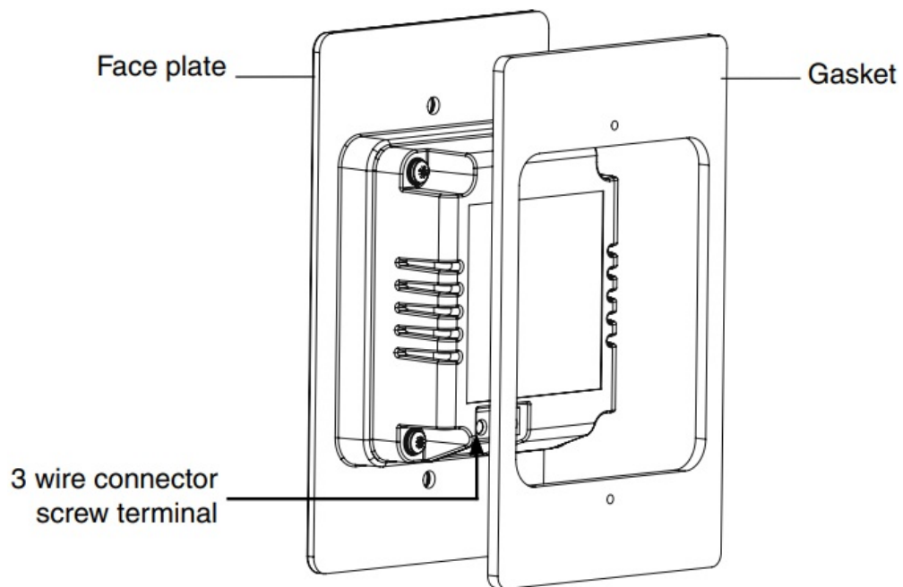
Controller Gasket Rear View
