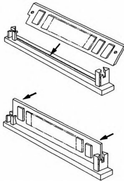
Installing SIMMs
