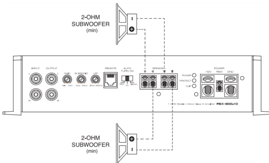
Fig.6 Two Single Voice Coil Subwoofer (2~4 ohms)
