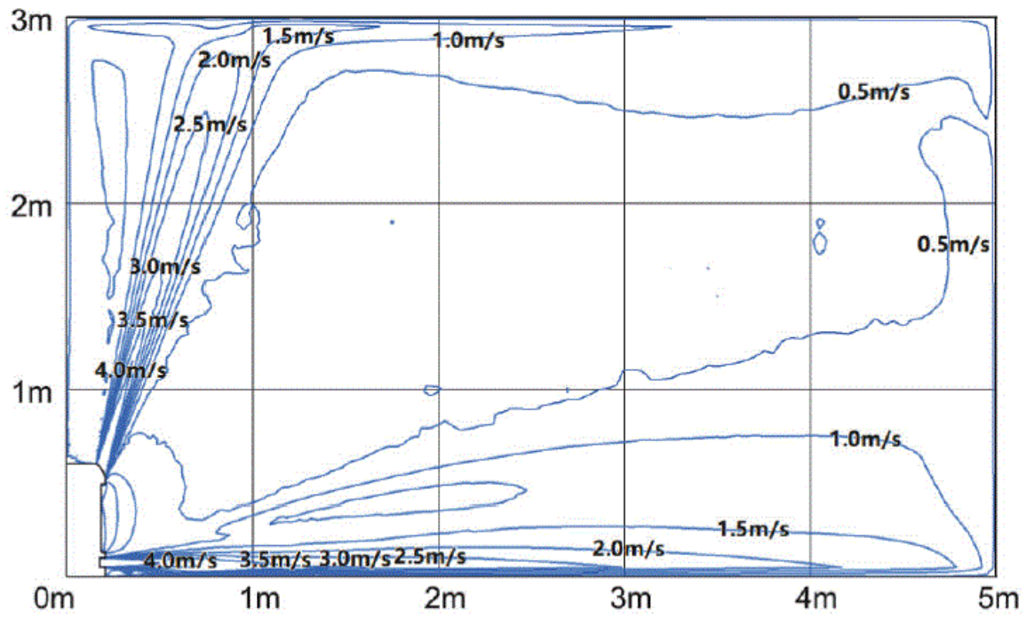
Fig. 11 – Cooling airflow velocity distributions
