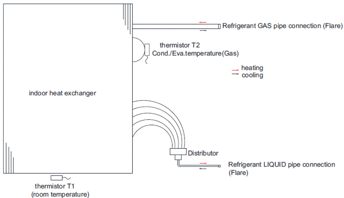
Fig. 16 – Refrigerant System Diagram
