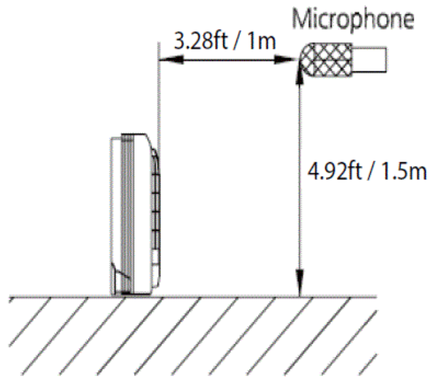
Fig. 7 – Sound Pressure Testing Method
