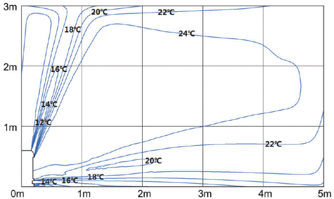
Fig. 12 – Cooling temperature distributions
