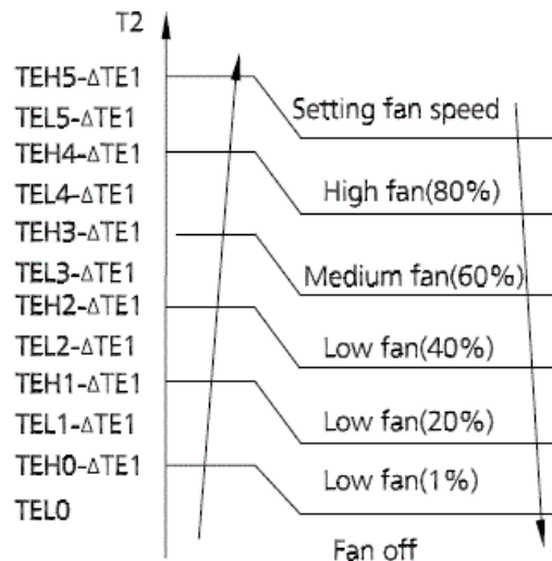
Fig. 20 – Anti-cold air function
