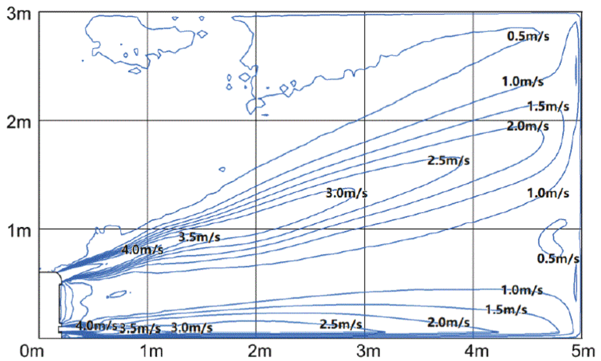
Fig. 13 – Heating airflow velocity distributions
