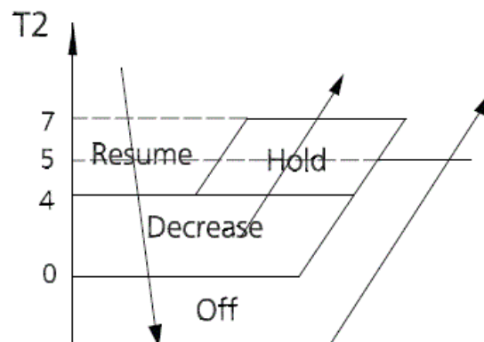
Fig. 19 – Evaporator Temperature Protection
