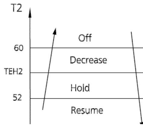
Fig. 21 – Evaporator Coil Temperature Protection
