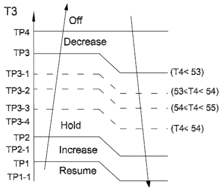
Fig. 18 – Condenser Temperature Protection
