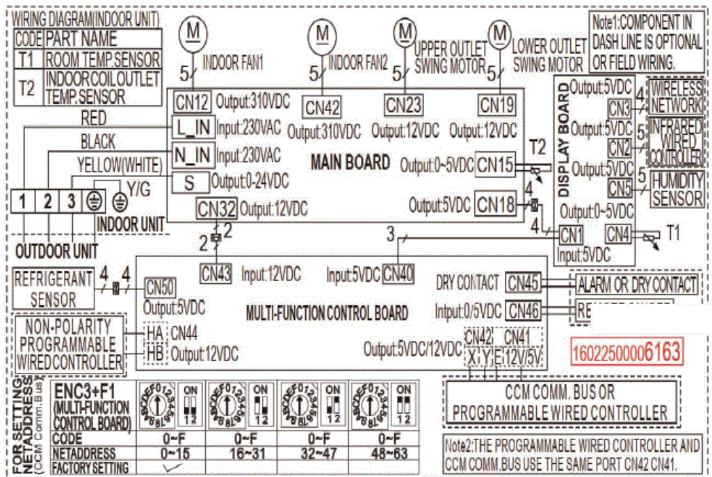
Fig. 15 – Wiring Diagram Sizes 09K, 12K, 16
