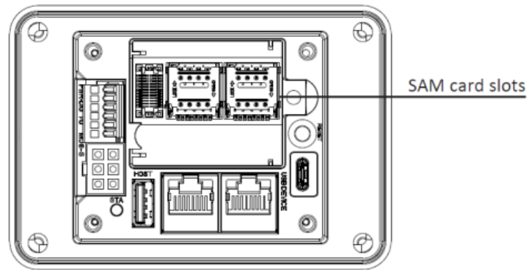
Figure 5: SAM card slots
