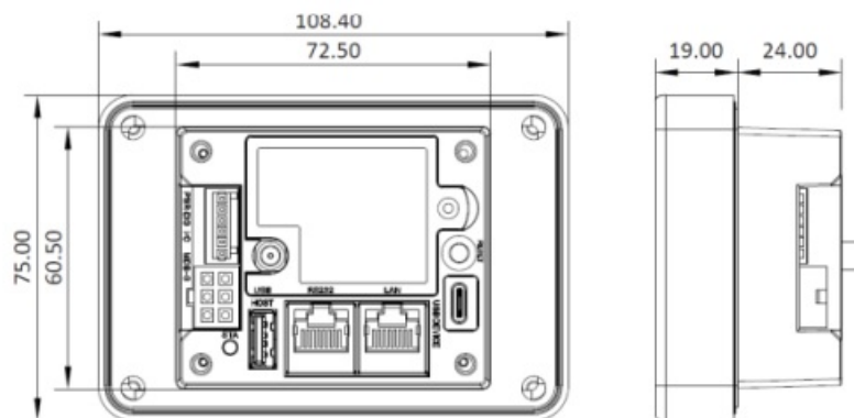
Figure 6: device dimensions (mm)
