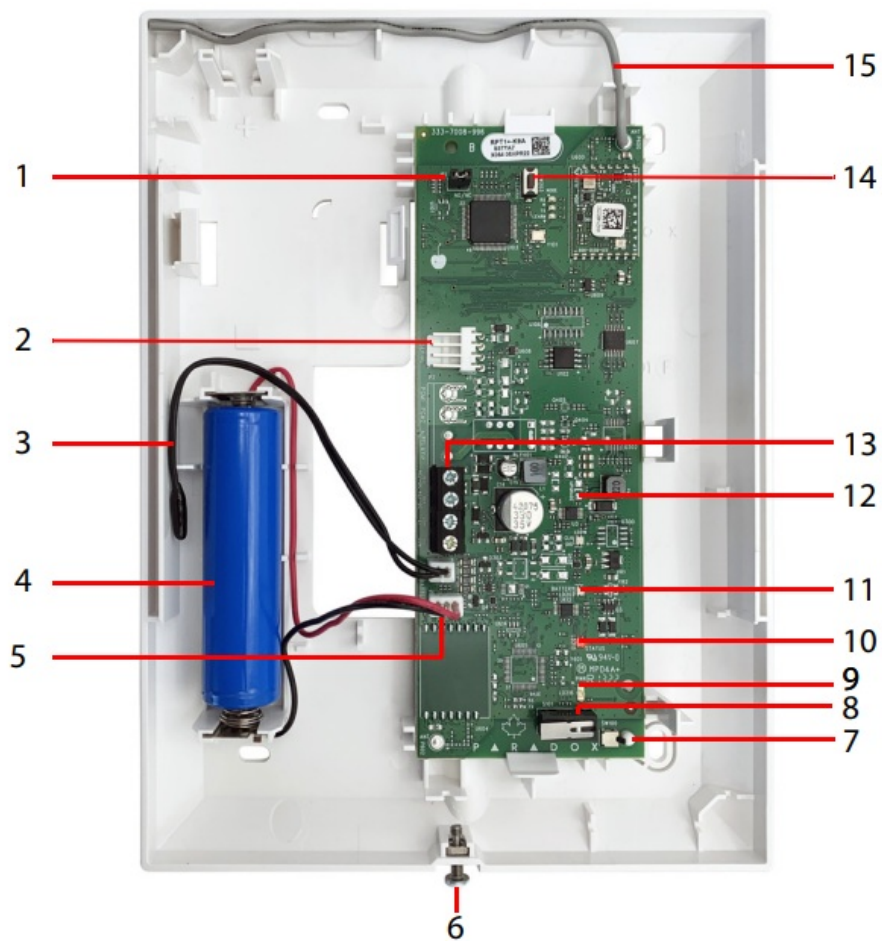
Figure 1: RPT1+ PCB
