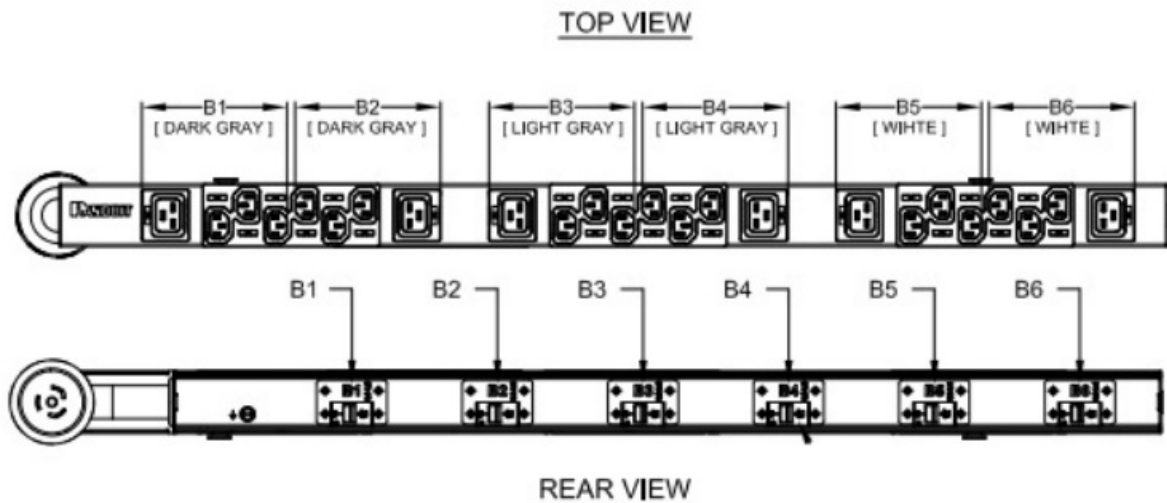
Three Phase Half-Height Dual-Sided PDU Example
