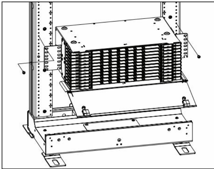
FlexCore™ Cassette Installation and Replacement (all cassettes sold separately)
