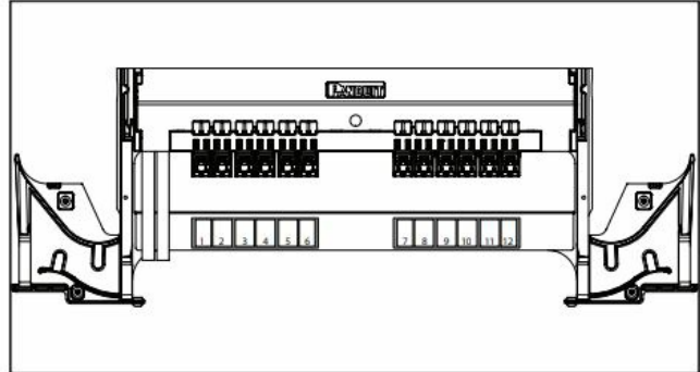
Fusion Splice Cassette with LC Adapters
