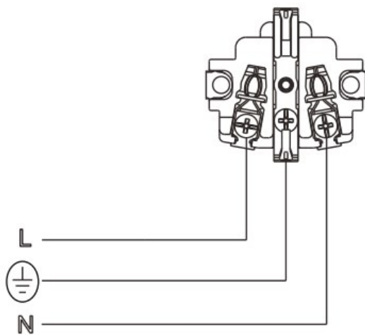
CIRCAUIT DIAGRAM
