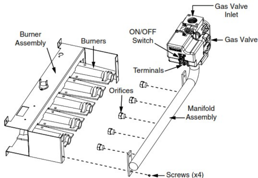
Figure 1. Typical Burner & Manifold Assembly
