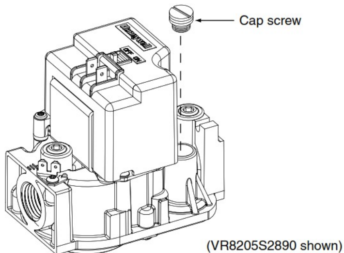
Figure 2. Cap Screw Removal
