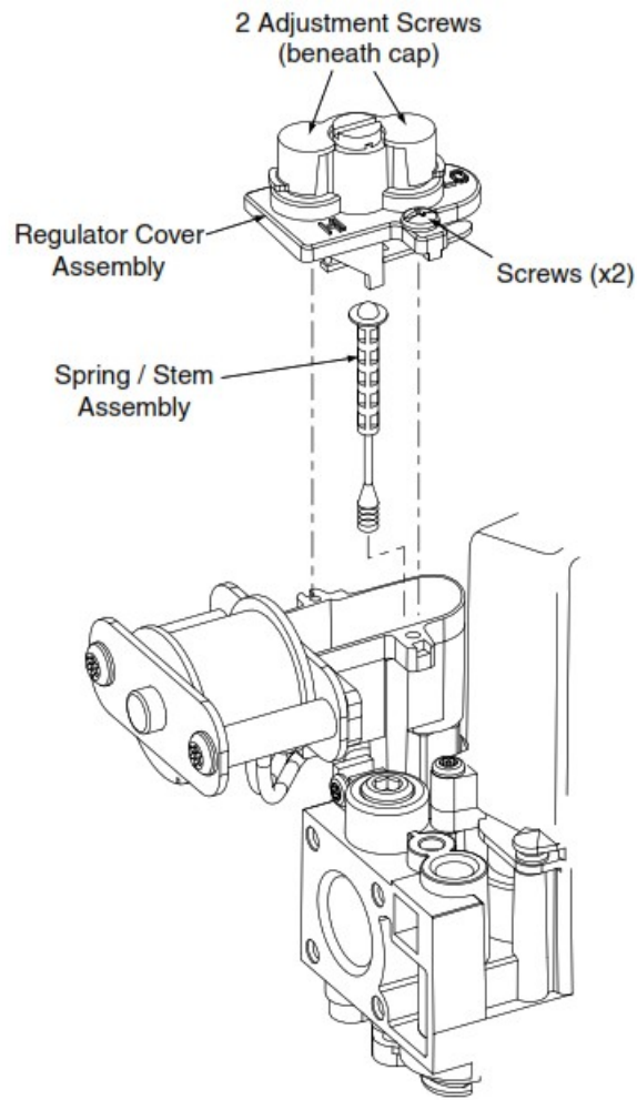
Figure 4. Spring / Stem Assembly Removal
