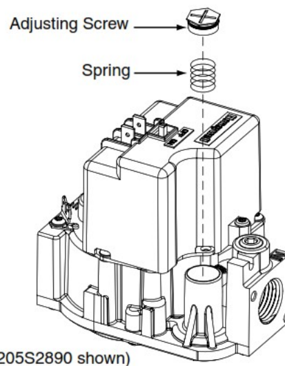
Figure 3. Pressure Regulator Spring & Adjustment Screw Removal
