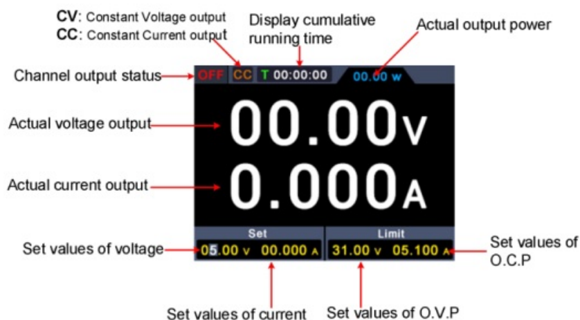
Figure 3-3 User Interface
