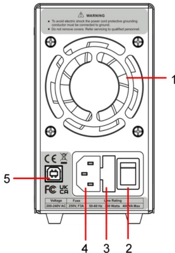
Figure 3-2 Rear Panel Overview
