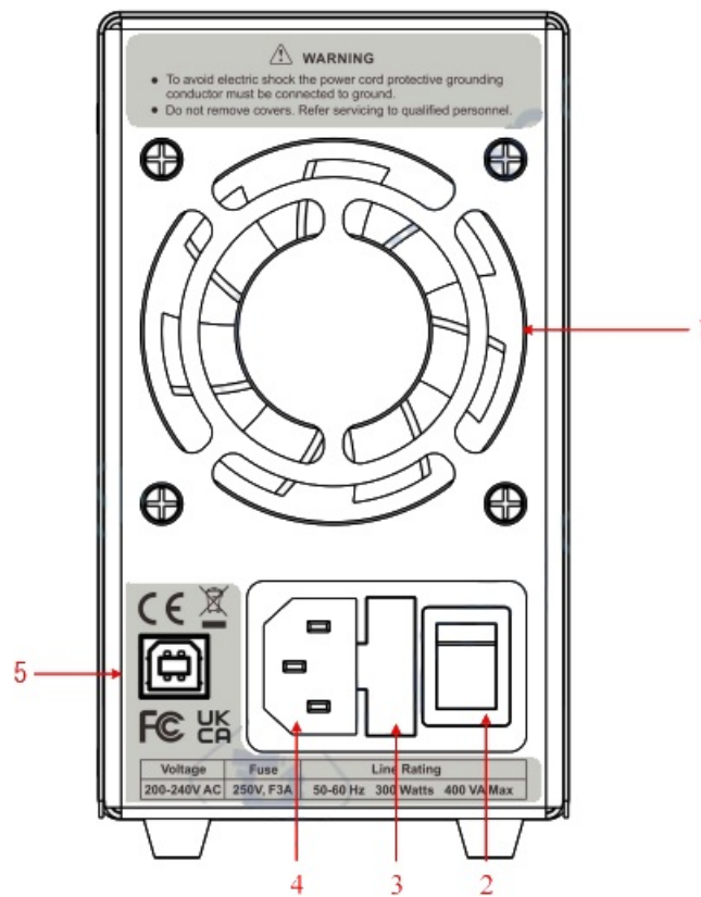
Figure 3-2 Rear Panel Overview
