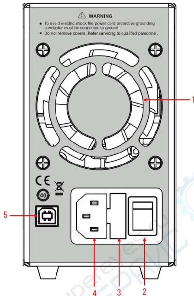
Figure 3-2 Rear Panel Overview
