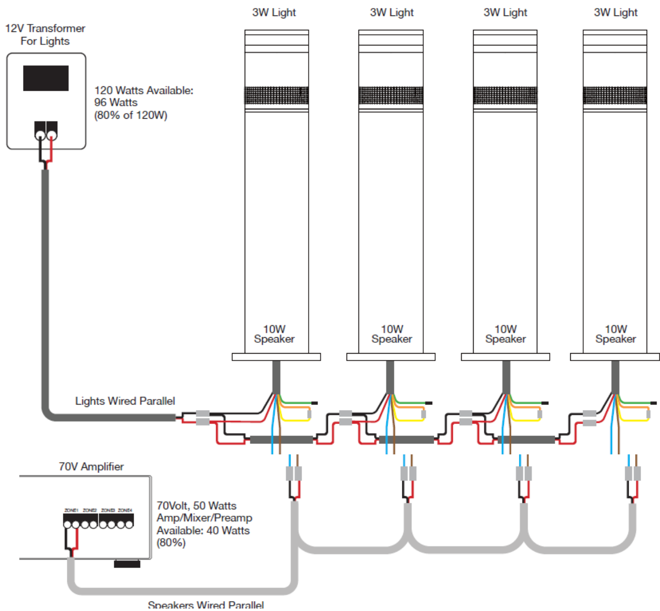
Eclipse25 WM – Right and Left 8-Ohm Stereo X 2pr = 4-ohm pair Sample System Diagram
