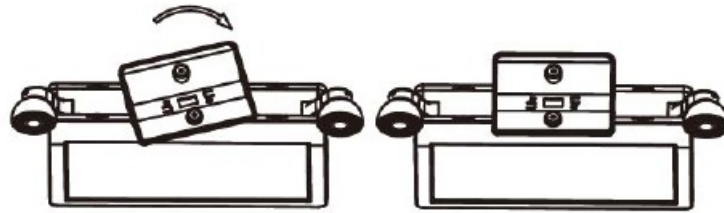
Fig.4 Canopy Assembly
