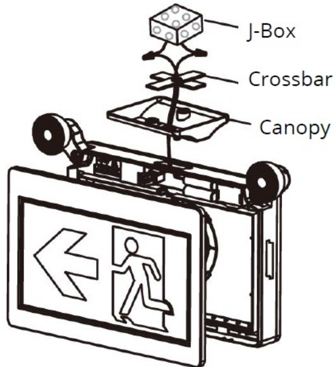
Fig.4 Canopy Assembly
