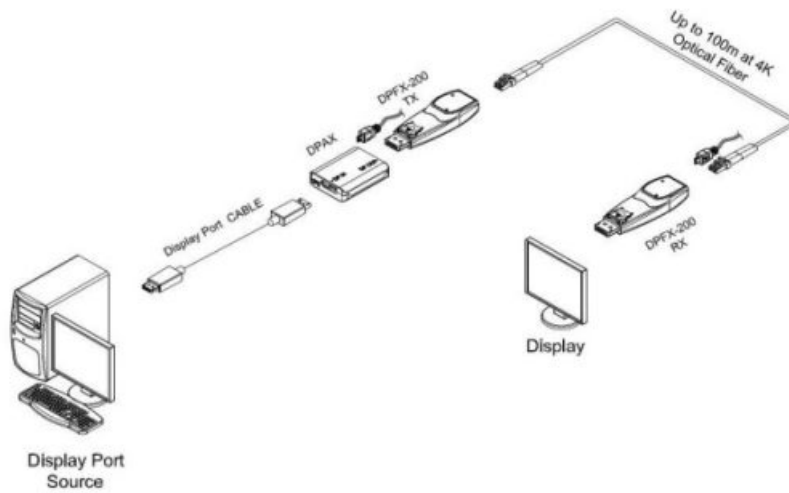
Figure 4 – Connection of DPAX with Copper cable and Optical fiber (TX side)
