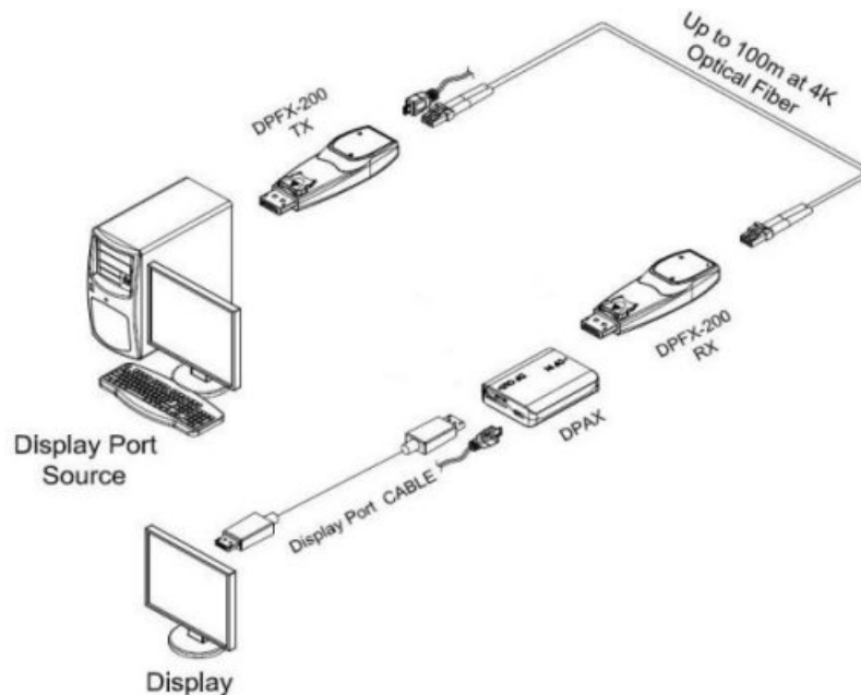
Figure 3 – Connection of DPAX with Copper cable and Optical fiber (RX side)
