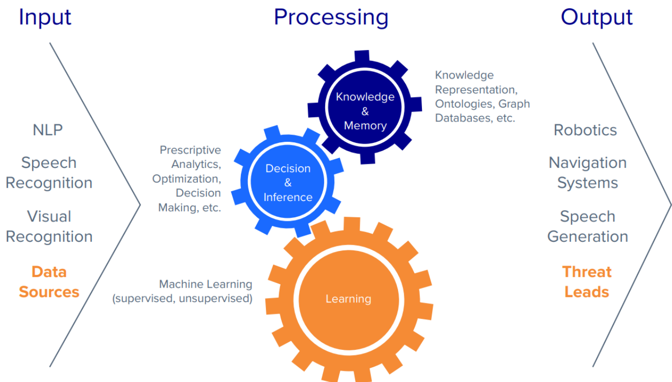
Figure 2. Artificial intelligence
