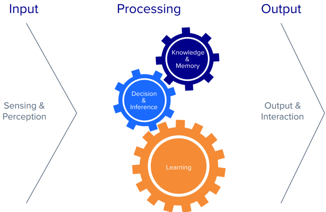
Figure 1. Human intelligence
