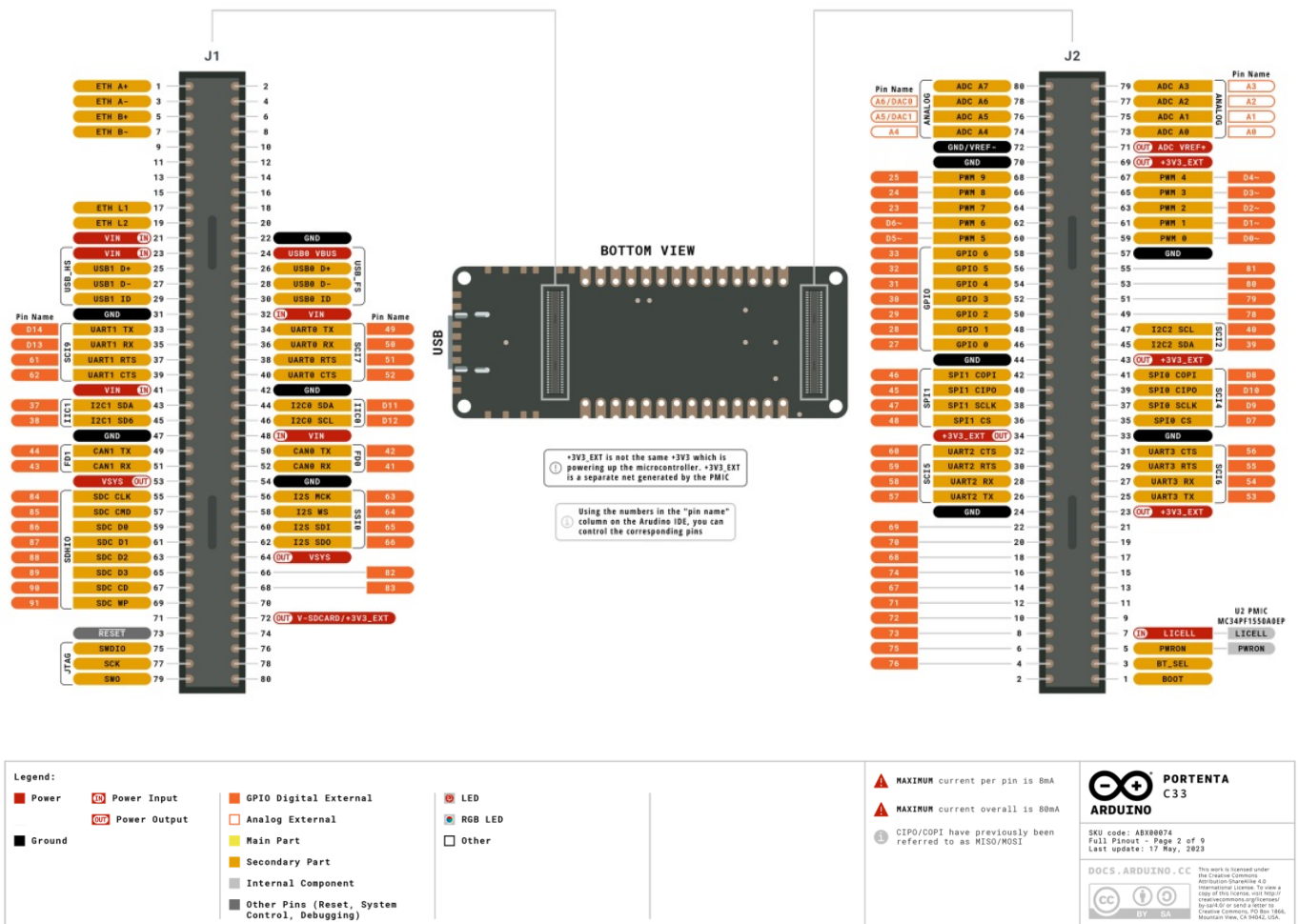
Figure 2. Portenta C33 pinout (High-Density connectors)
