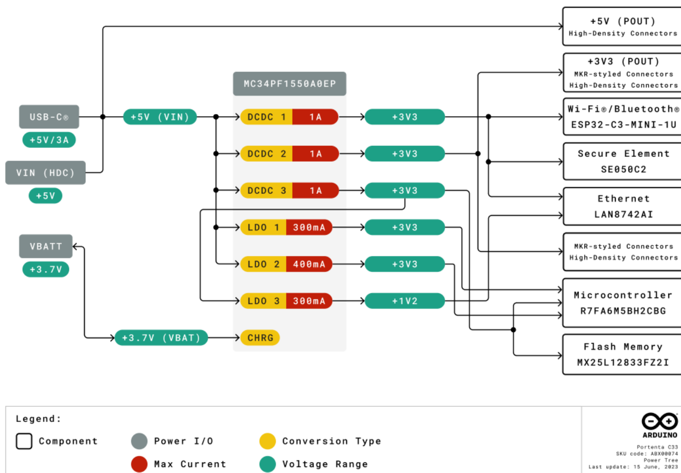
Figure 4. Power architecture of the Portenta C33
