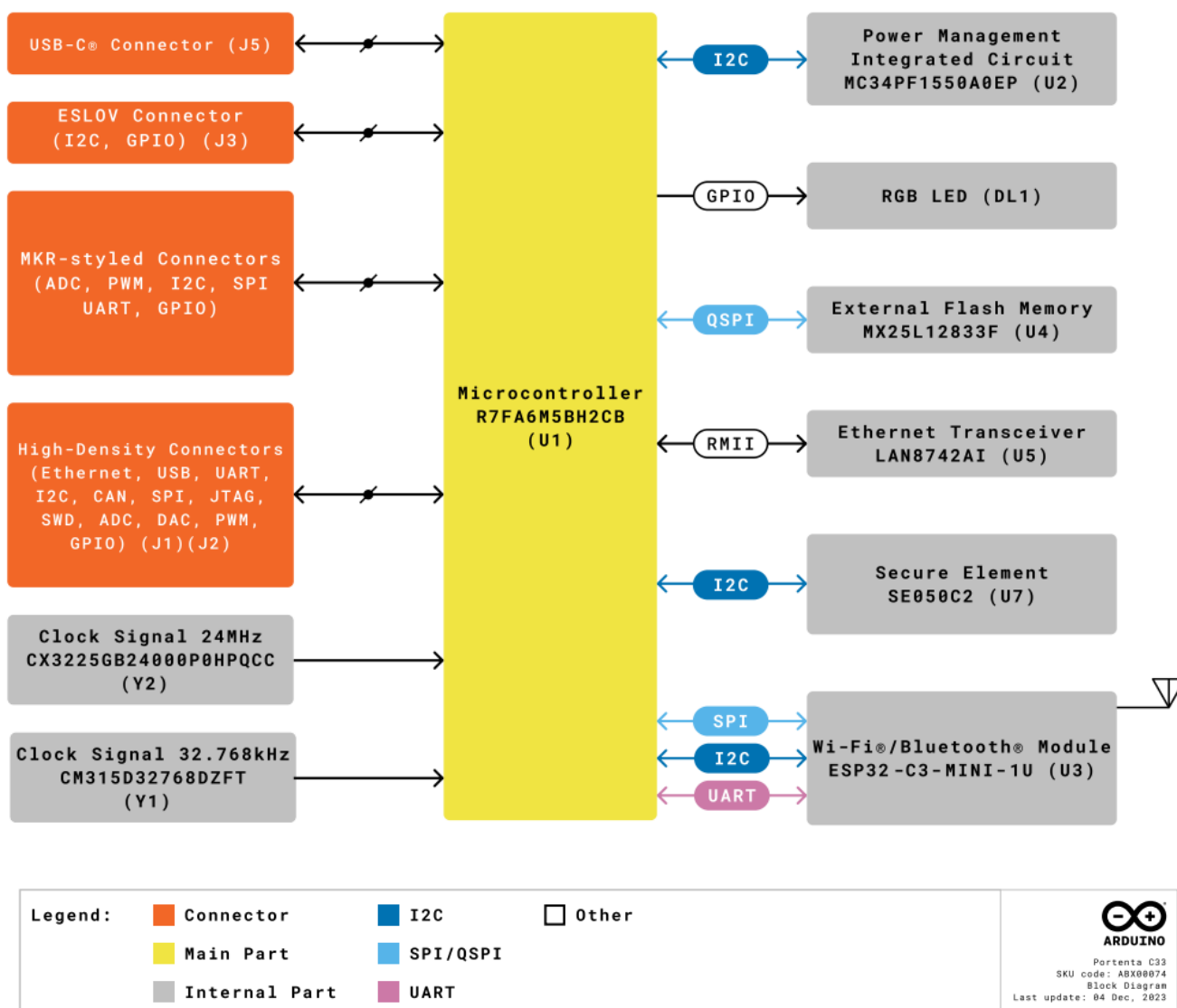
Figure 3. High-level architecture of the Portenta C33
