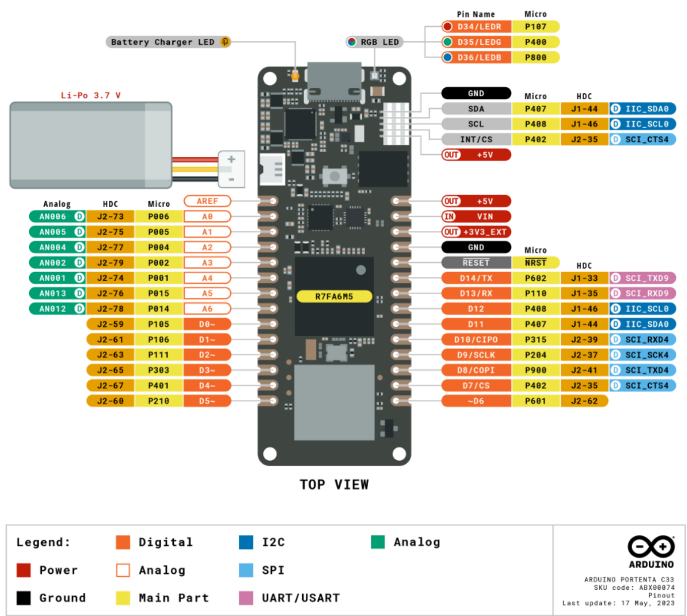
Figure 1. Portenta C33 pinout (MKR-styled connectors)
