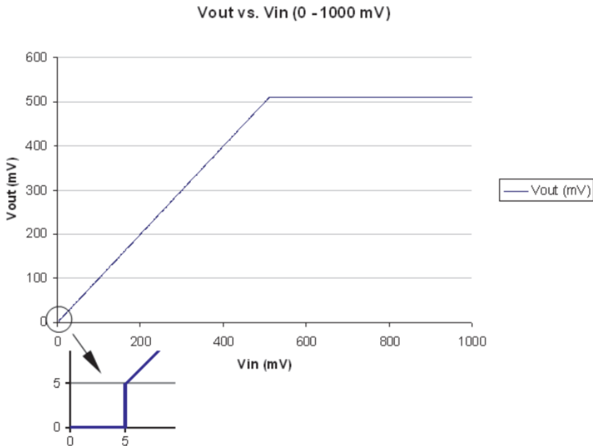
Minimum Input Voltage Graph
