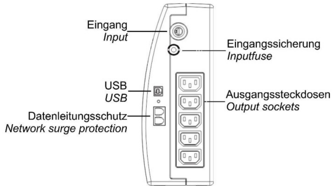
Figure 5: Rear view of YUNTO 1200 - 1500
