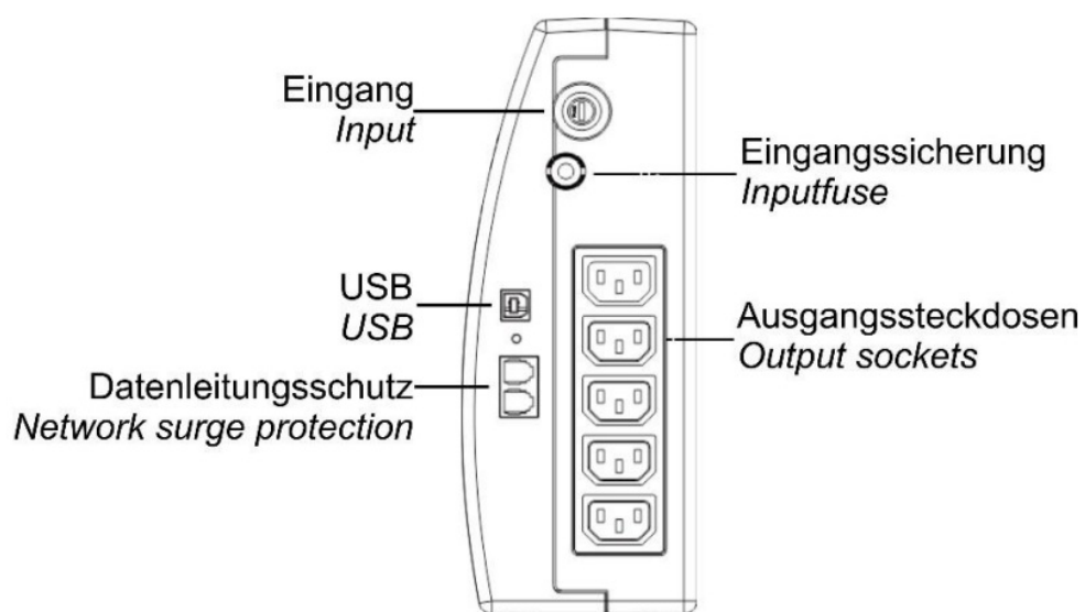
Figure 5: Rear view of YUNTO 1200 - 1500
