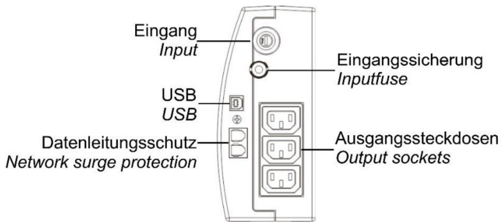
Figure 4: Rear view of YUNTO 500 - 800
