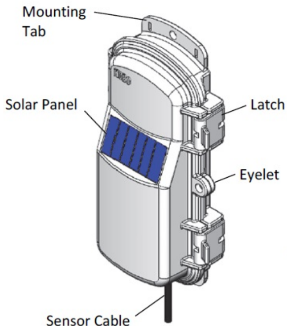
Sensor Mote Closed, Front
