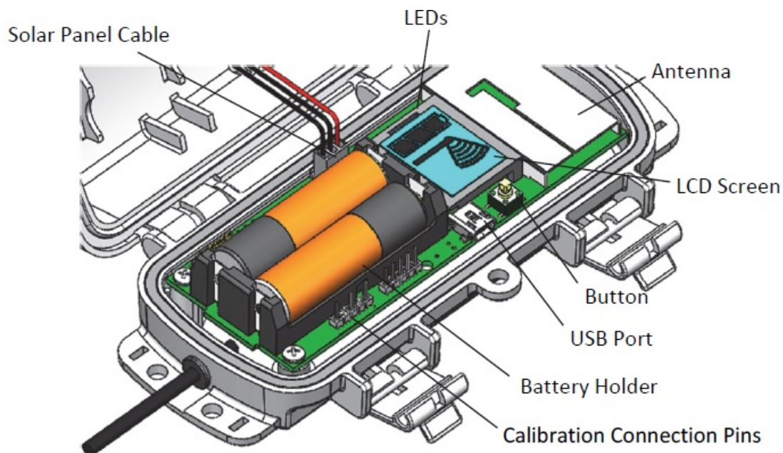
Sensor Mote Opened
