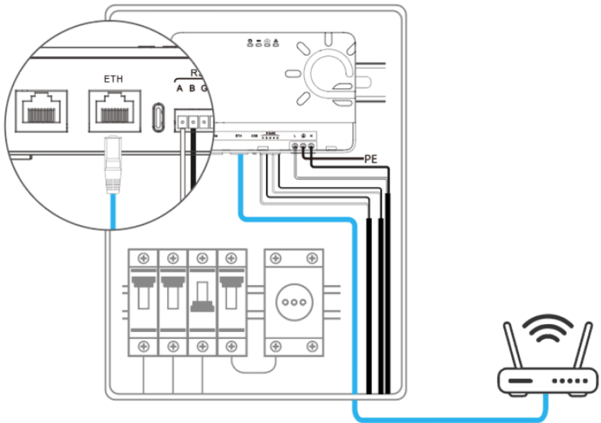
Fig. 4 diagram of Ethernet connection
