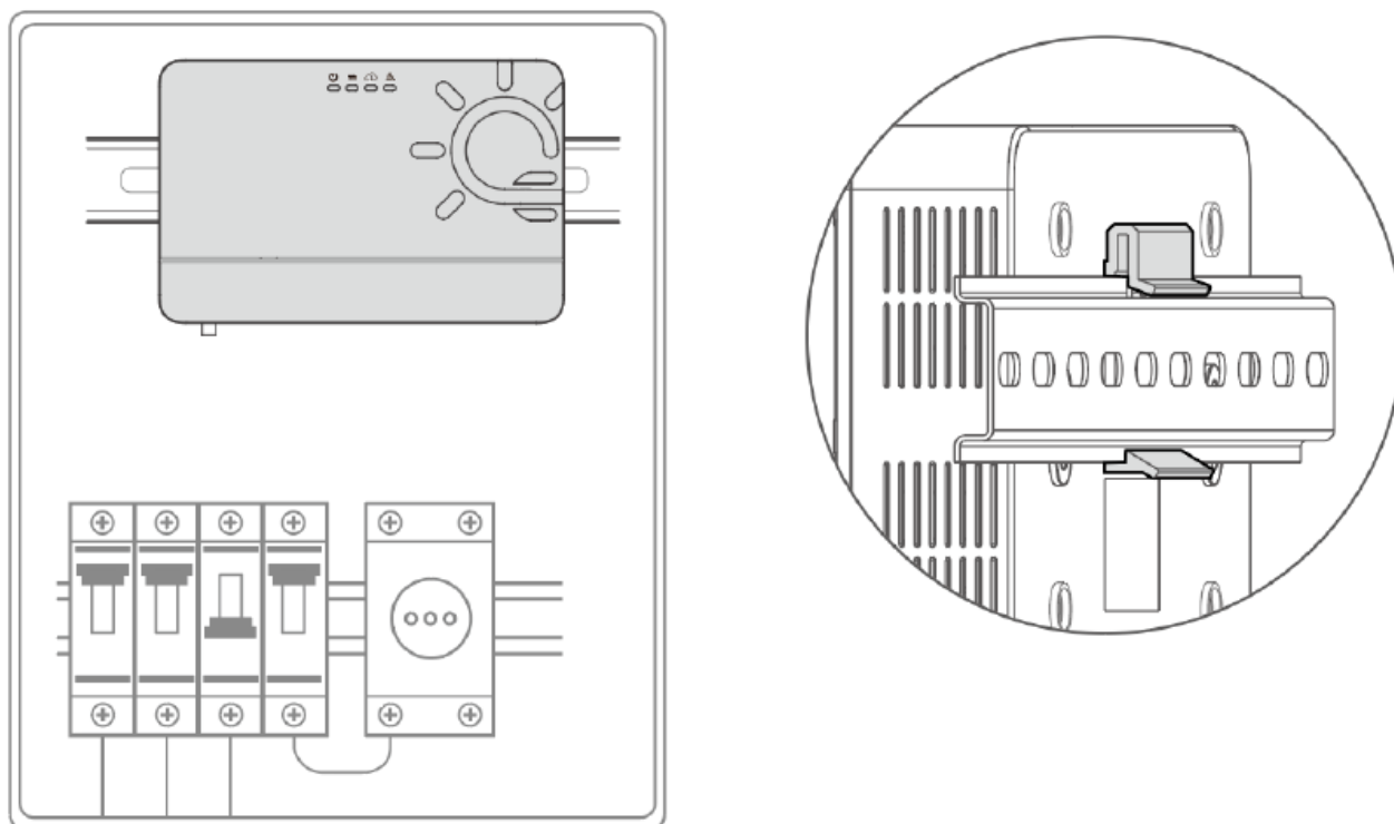
Figure 2. Installation of EQ-MU-Pro
