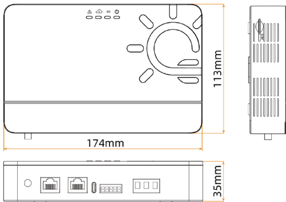
Figure 4eq-mu-pro size chart
