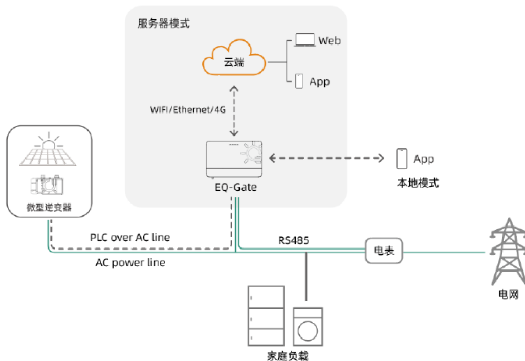
FIGURE-2EQ-MU-PRO communication topology
