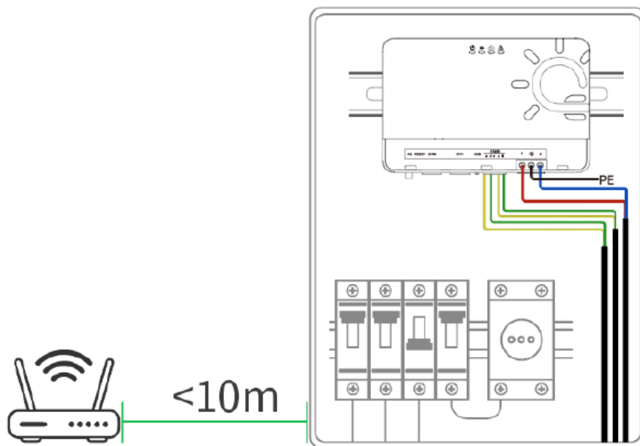
Figure-5 installation distance diagram
