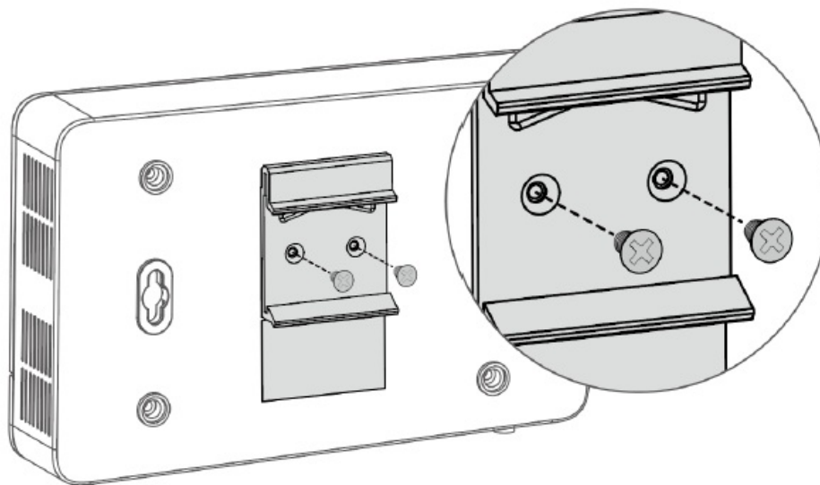
Fig. 1 schematic diagram of mounting guide rail buckle
