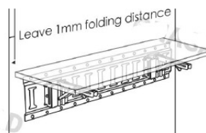
STEP 3: Place the board on top
