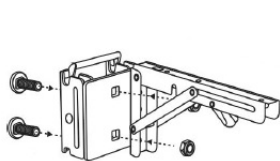
STEP 1: Assemble with bolts and nuts
