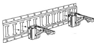
STEP 2: Snap them into the anchor points of E track
