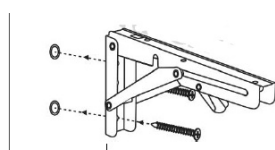
STEP 4: Put the long screws through the brackets and install them
