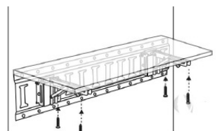
STEP 4: Tighten and secure the board with the short screws
