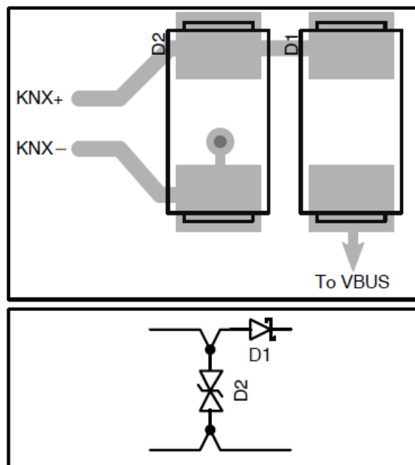
Figure 20. Optimal Layout for the TVS Diode
