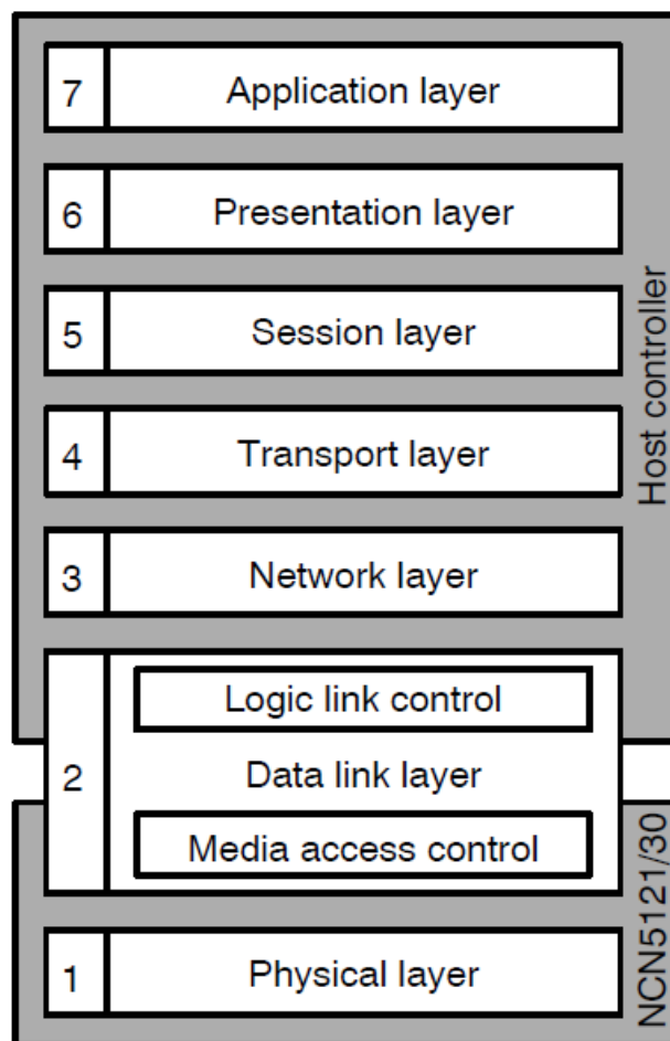
Figure 10. Placement of the Transceivers in the OSI Model
