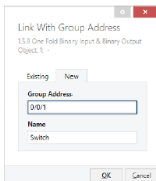
Figure 35. Assign a New Group Address
