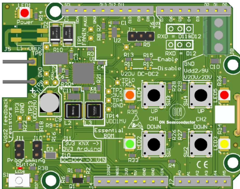
Figure 2. NCN5100AS-2 Evaluation Board
