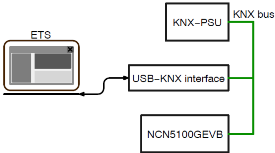
Figure 23. Minimal Network Setup
