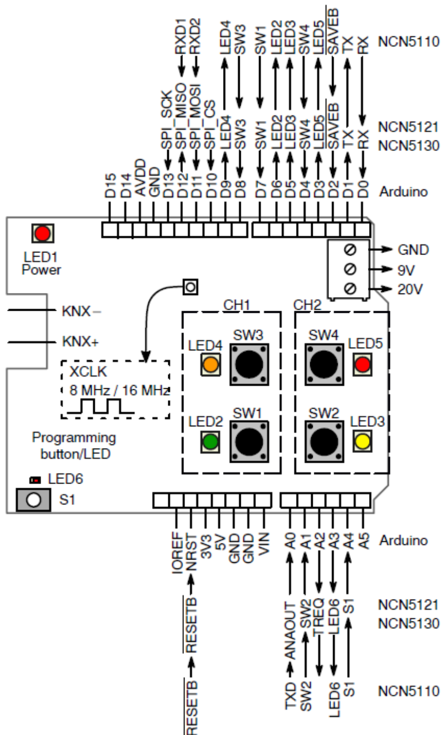
Figure 9. Evaluation Board Connectivity (KNX-Shield)
