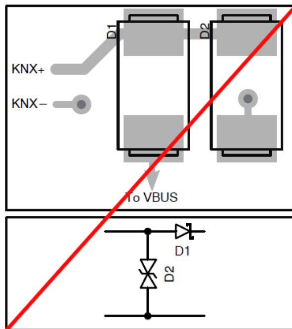
Figure 19. Wrong Layout for the TVS Diode
