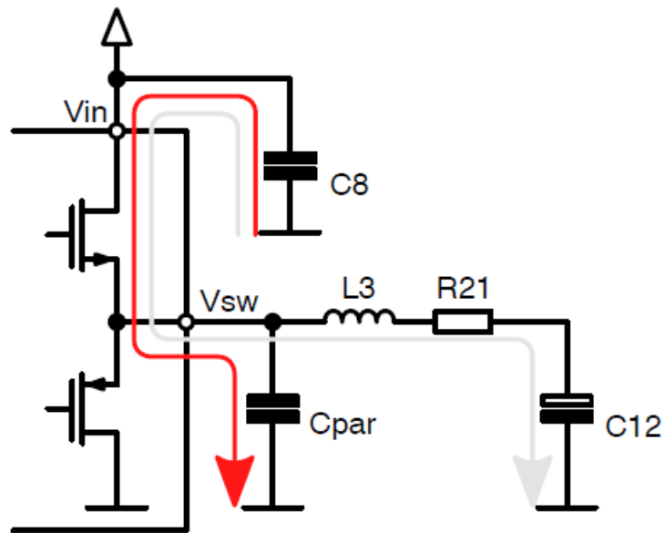
Figure 17. Schematic Showing the DC-DC Converter Current Loops
