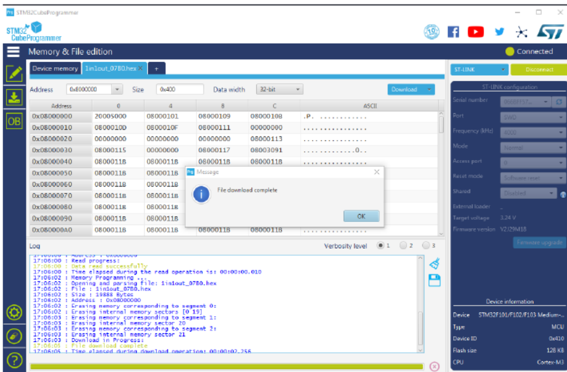
Figure 30. Program the Nucleo Using the STM32CubeProgrammer
