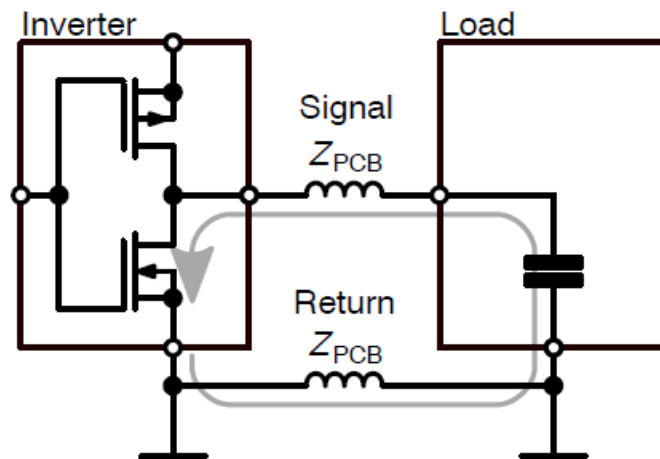
Figure 15. Optimizing the Return Path in a Dual-layer Design
