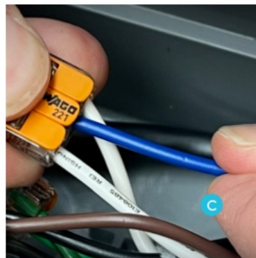
Wire the New Power Supply
