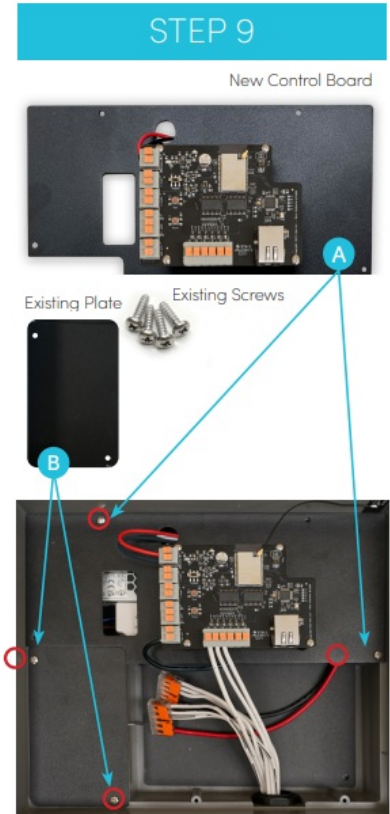
Attach the Above Plates
