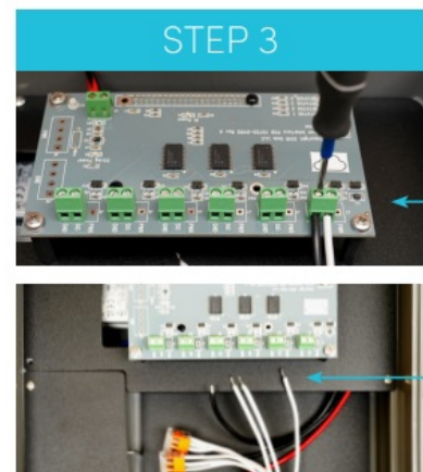
Disconnect PCB Wires
