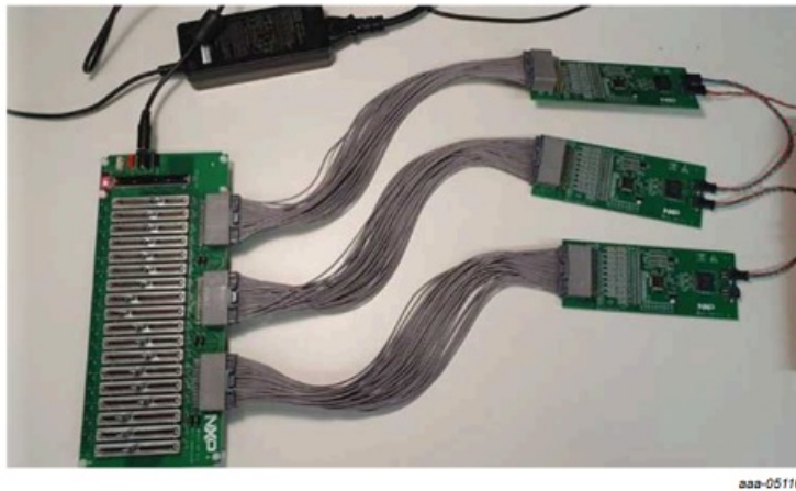
Figure 6. RD33774PDSTEBs connection to a BATT-18EMULATOR
