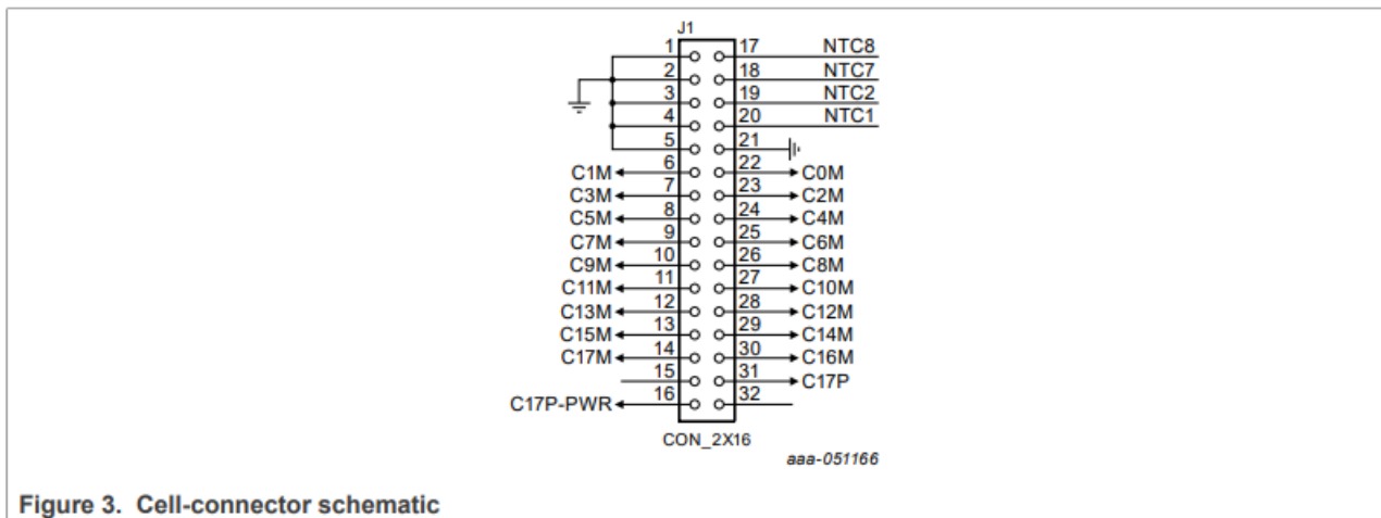
Figure 3. Cell-connector schematic
