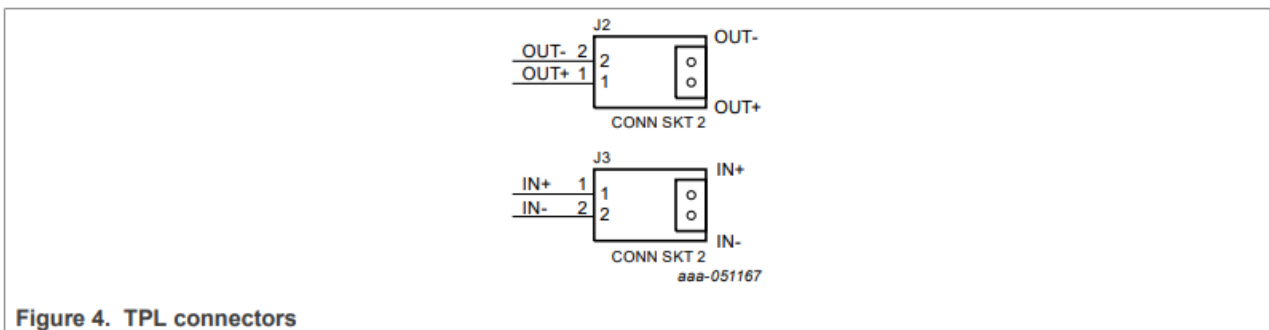
Figure 4. TPL connectors
