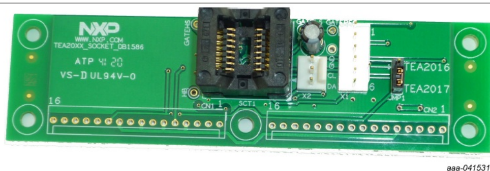
Figure 2. TEA20xx_SOCKET_DB1586 programming board (SO16 socket)
