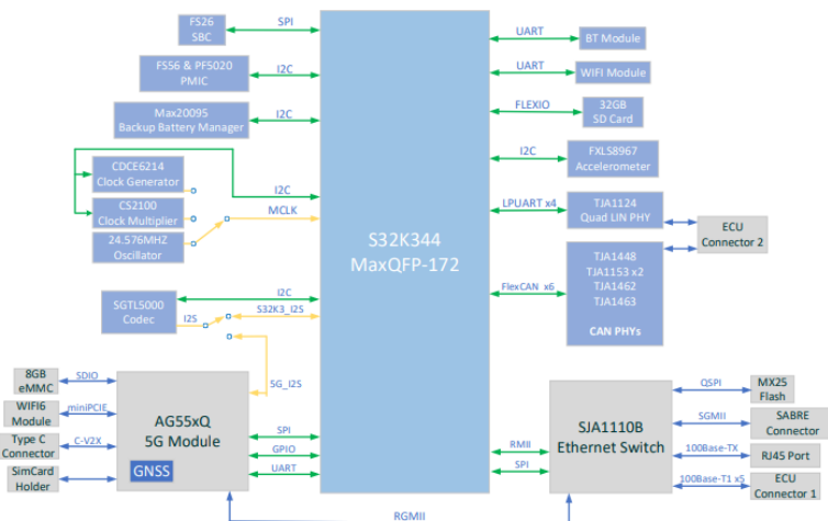
Figure 1. the Block Diagram
