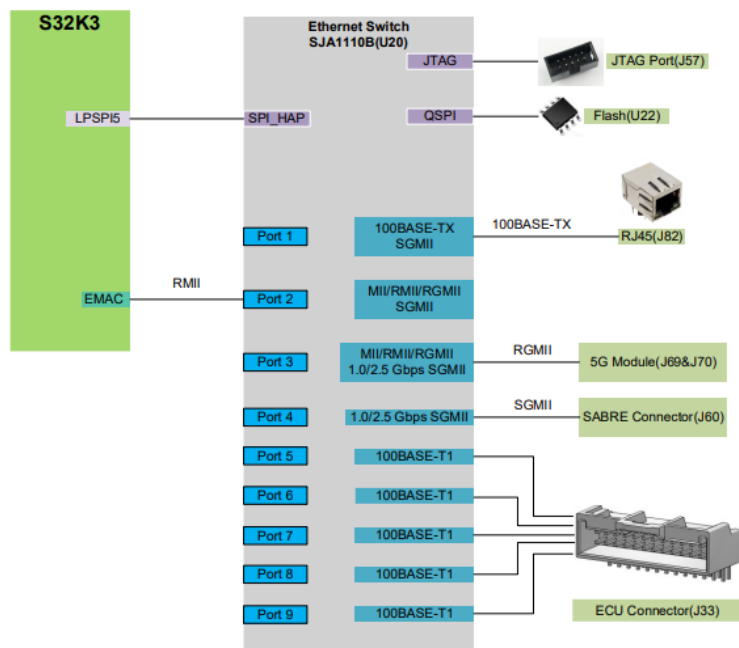
Figure3. the Ethernet Switch SJA1110B Block Diagram
