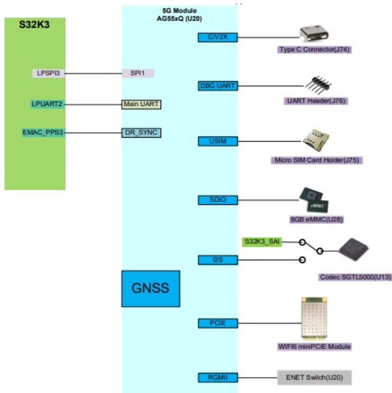
Figure4. the 5G Module Diagram
