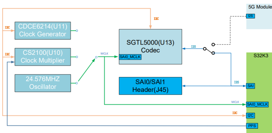
Figure5. the AVB Hardware Diagram
