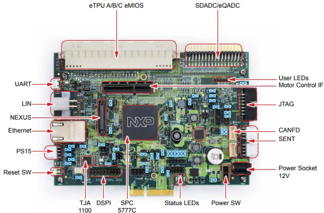
Figure 1: Top elevation of MPC5777C Development Board
