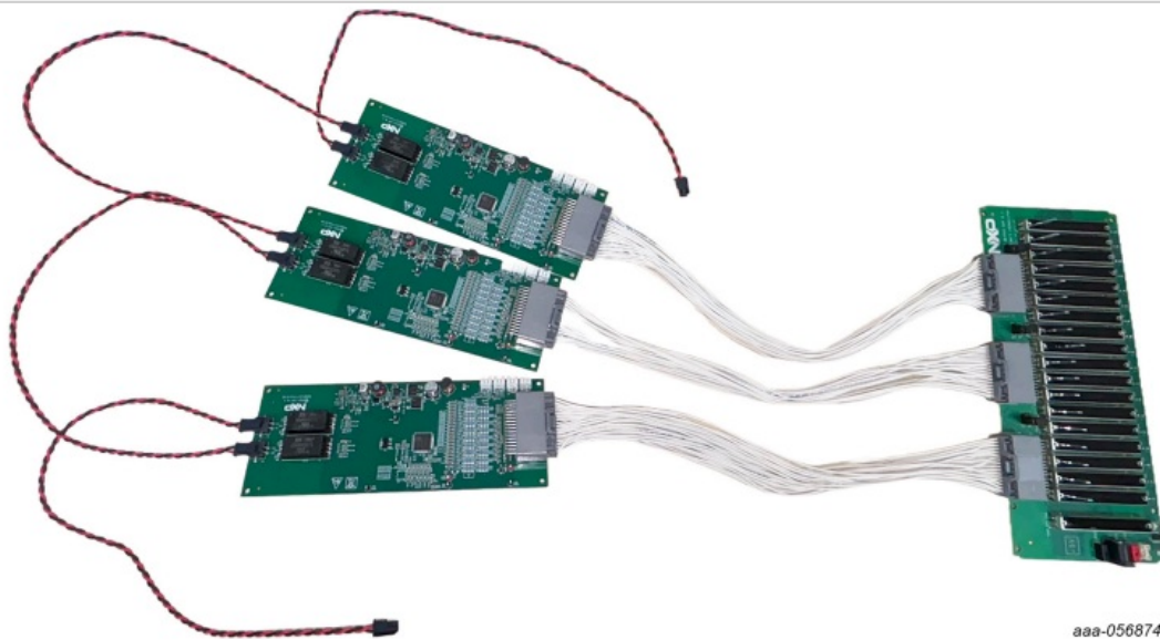
Figure 10. Battery emulator connection
