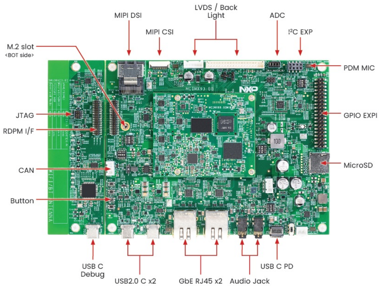
Figure 1: Top view i.MX 93 11x11 EVKPF09 board
