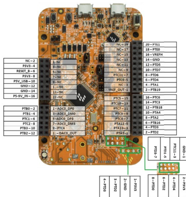
Figure 17. FRDM-K22F I/O header pinout
