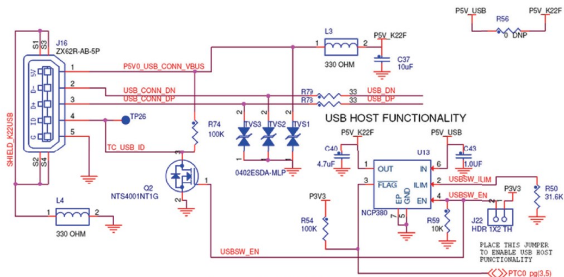
Figure 8. K22F USB port
