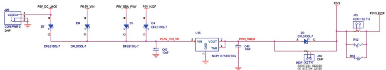
Figure 3. Power supply schematic
