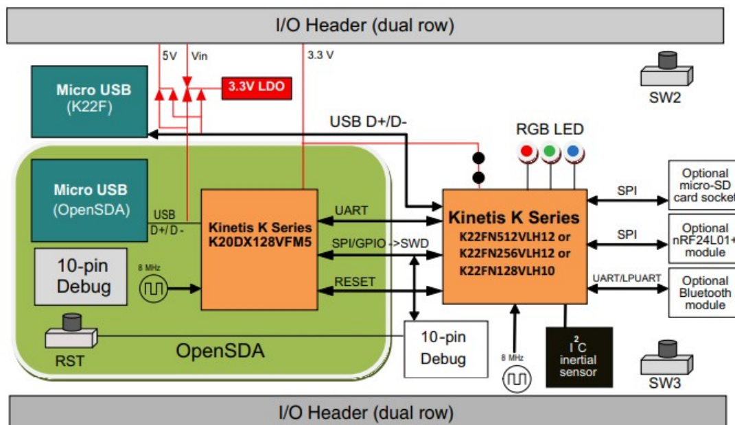
Figure 1. FRDM-K22F block diagram
