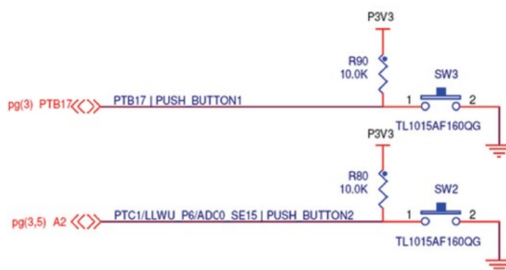
Figure 14. Push button switches
