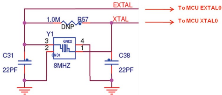
Figure 6. 8 MHz crystal clock source for MCU
