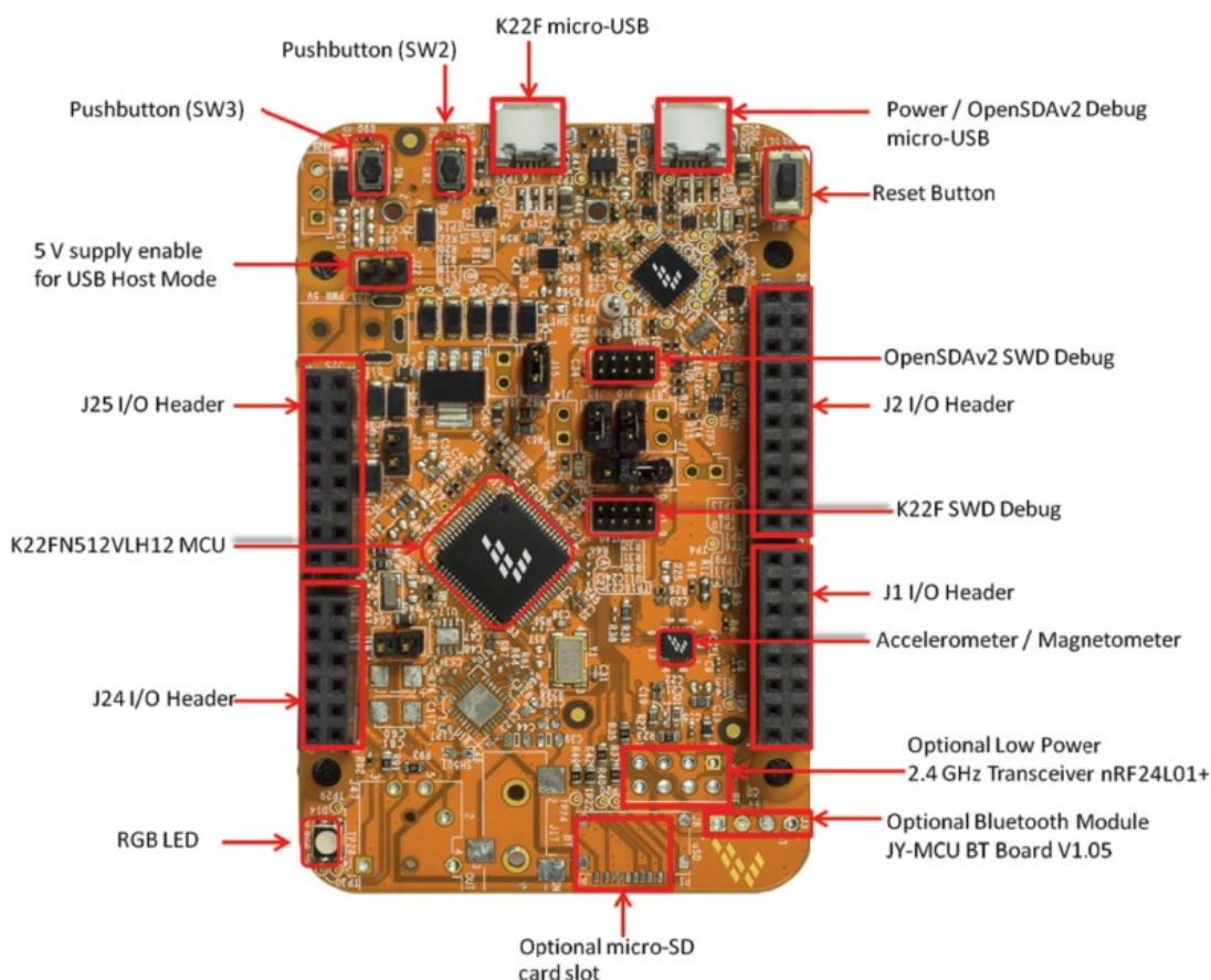
Figure 2. FRDM-K22F primary component placement
