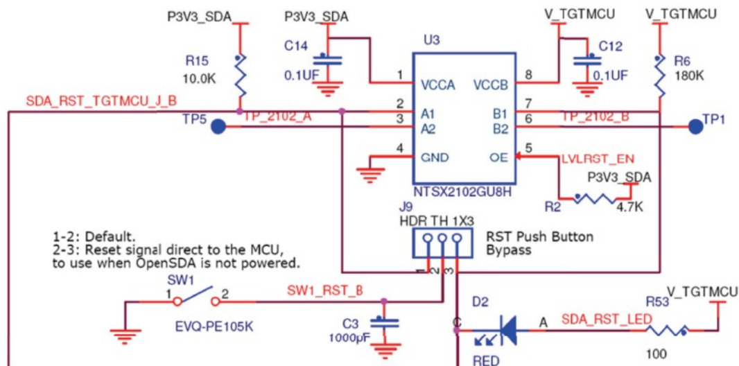
Figure 13. Reset circuit
