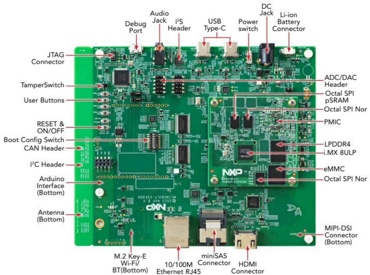
Figure 1: Main interfaces of i.MX 8ULP EVK9
