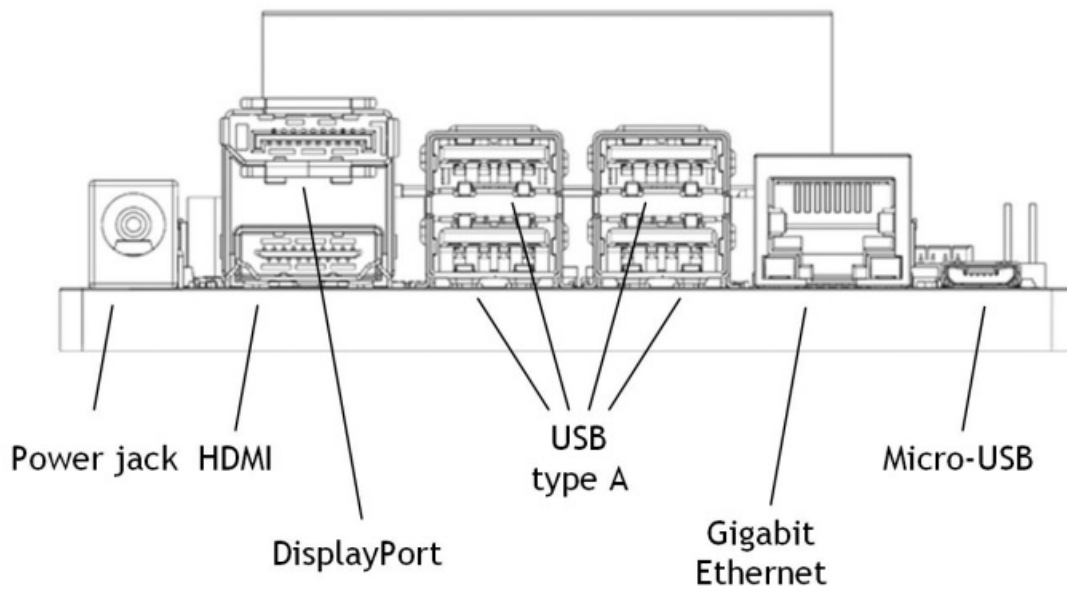
Developer kit module and carrier board: rear view
