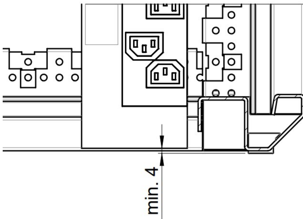
Power cable at TOP
