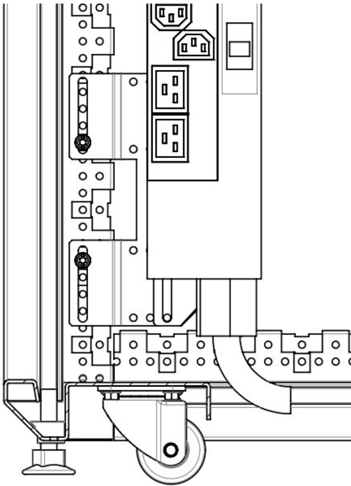
HEAVY LOAD CROSS BAR 19 ''
