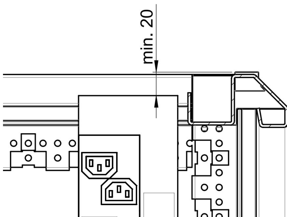
DEPTH MEMBER FIXING
