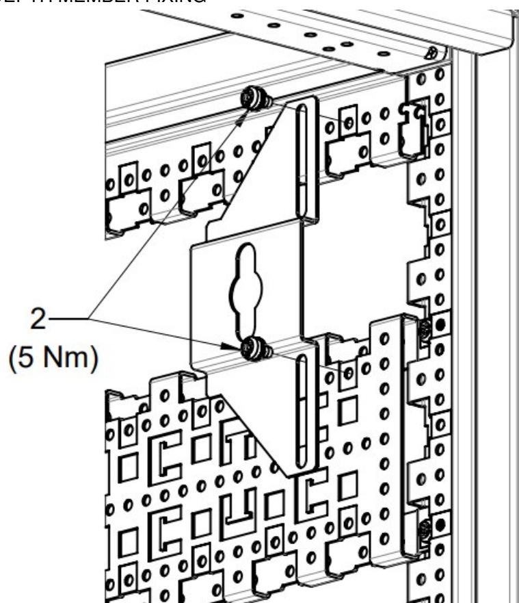
DEPTH MEMBER FIXING
