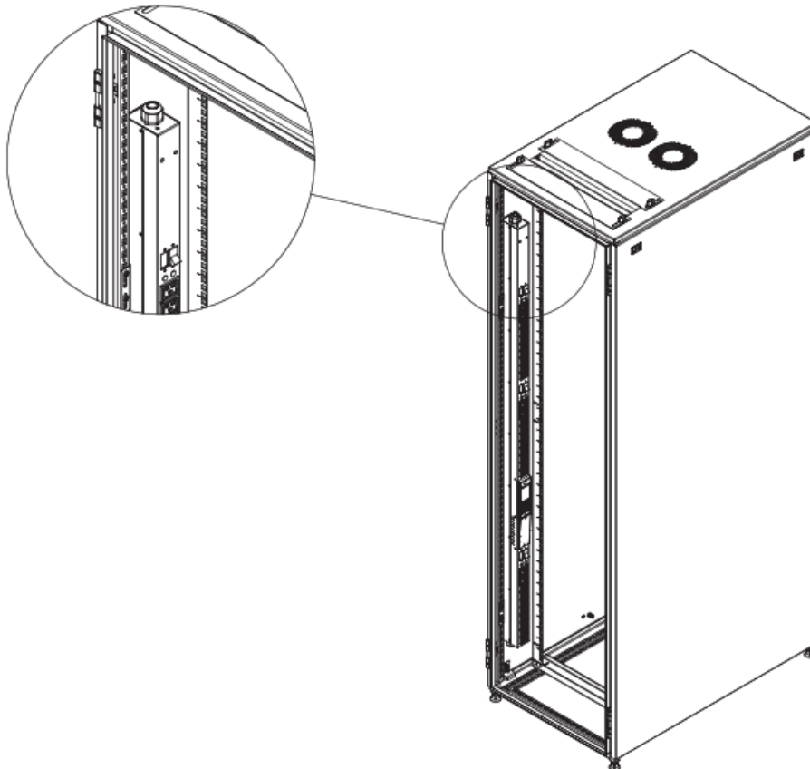
Frame Mount, Dual Feed PDU, Inward Facing
