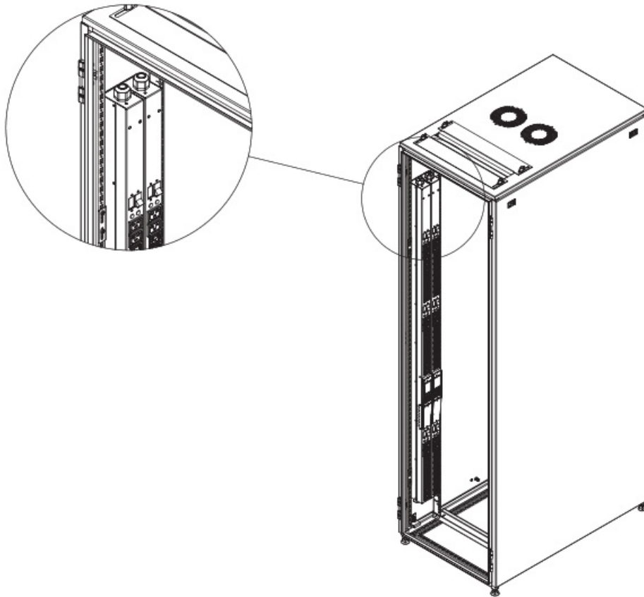
Frame Mount, Dual Feed PDU, Inward Facing
