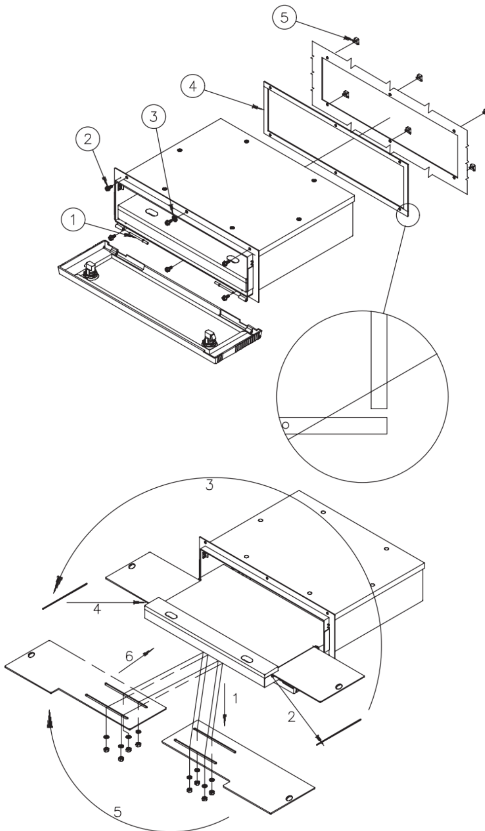
Reversing Mouse Tray, 600 mm Only
