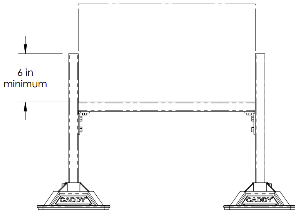
Configuration of conduit/pipe supply
