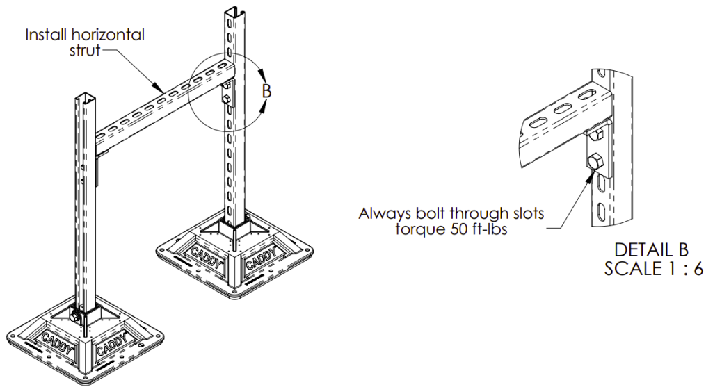
Configuration of pipe hanging
