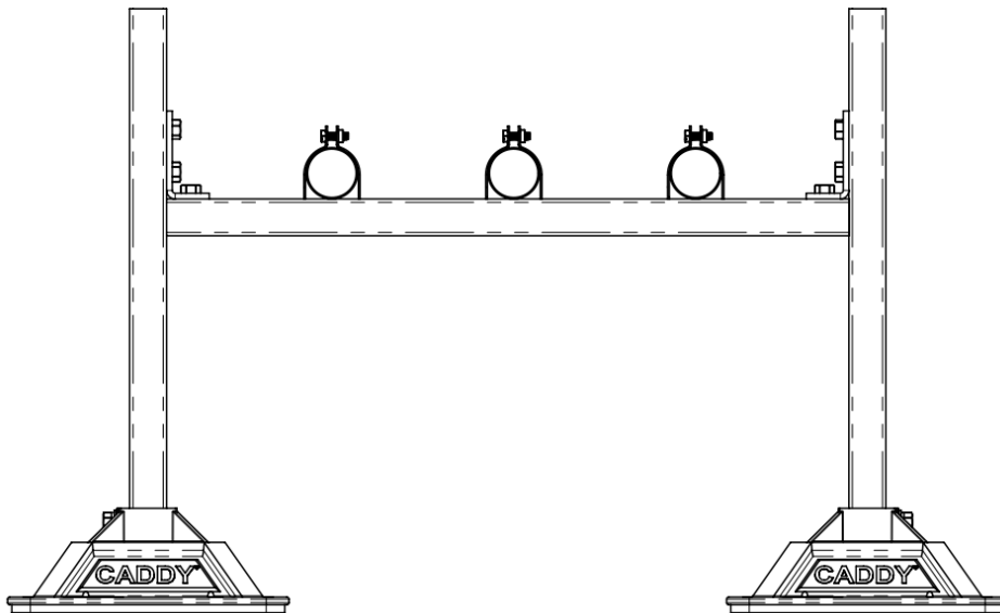
Configuration of conduit/pipe supply
