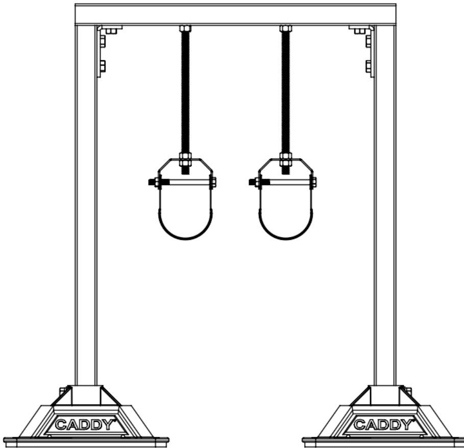
Configuration of pipe hanging
